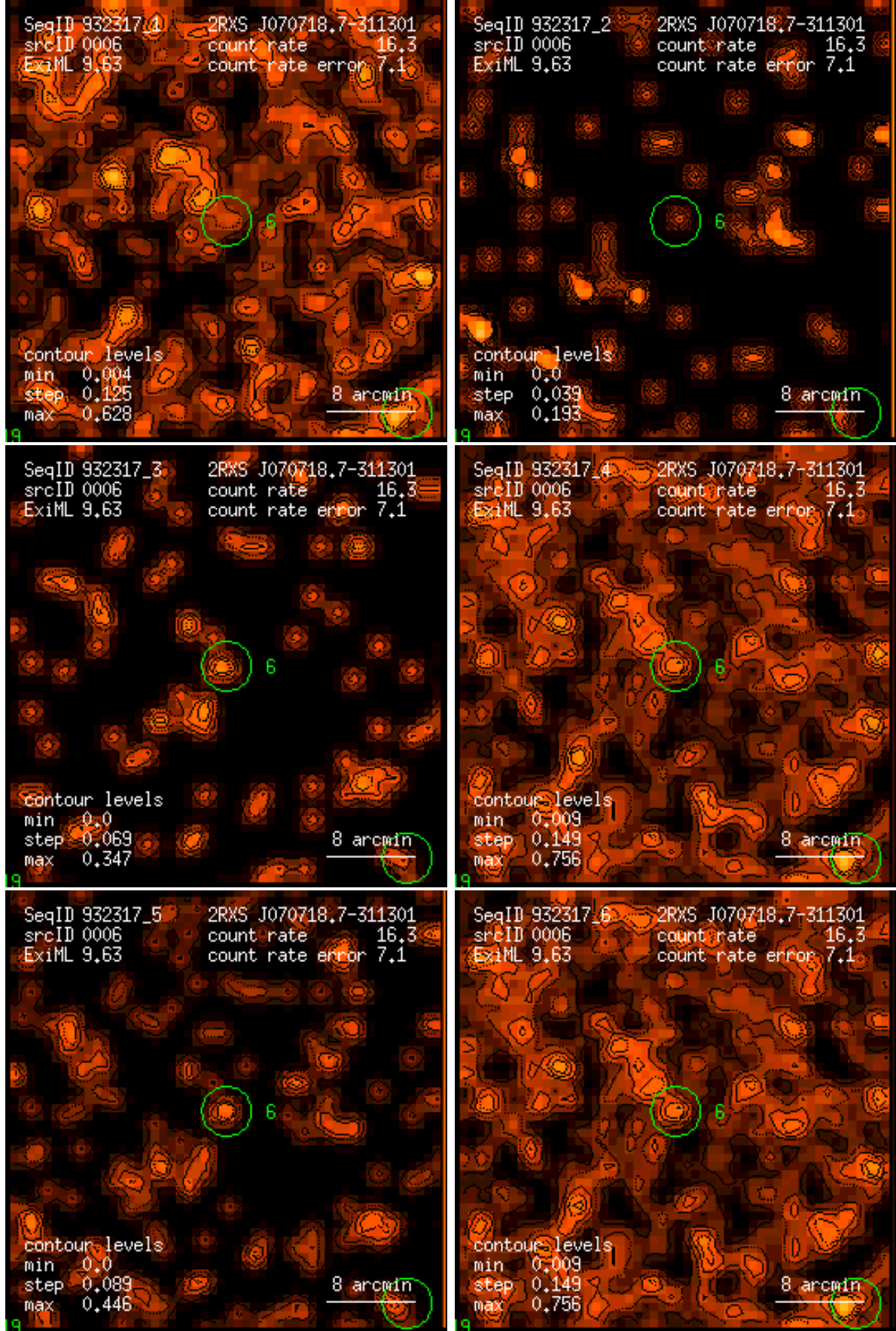
Figure 6: RASS 932317: detection 0006: band rate images, Gaussian filter: (1) PSPC channels 11 – 41, (2) 52 – 90, (3) 91 – 201, (4) 11 – 235, (5) 52 – 201, (6) 11 – 201. Broad band rates in counts/ks. Band rate contour levels in counts/ks/arcmin 2 .
