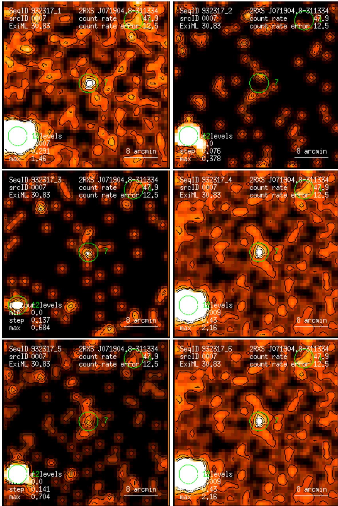
Figure 7: RASS 932317: detection 0007: band rate images, Gaussian filter: (1) PSPC channels 11 – 41, (2) 52 – 90, (3) 91 – 201, (4) 11 – 235, (5) 52 – 201, (6) 11 – 201. Broad band rates in counts/ks. Band rate contour levels in counts/ks/arcmin 2 .
