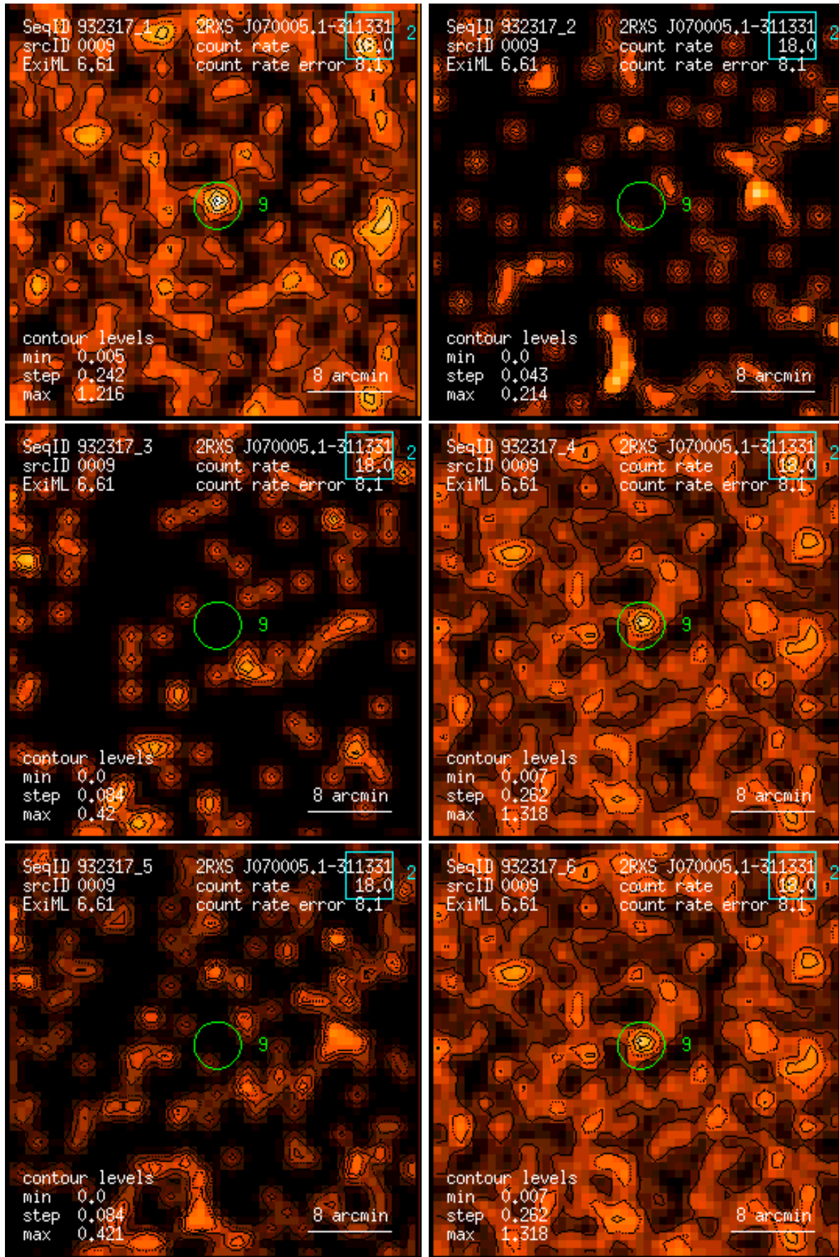
Figure 9: RASS 932317: detection 0009: band rate images, Gaussian filter: (1) PSPC channels 11 – 41, (2) 52 – 90, (3) 91 – 201, (4) 11 – 235, (5) 52 – 201, (6) 11 – 201. Broad band rates in counts/ks. Band rate contour levels in counts/ks/arcmin 2 .
