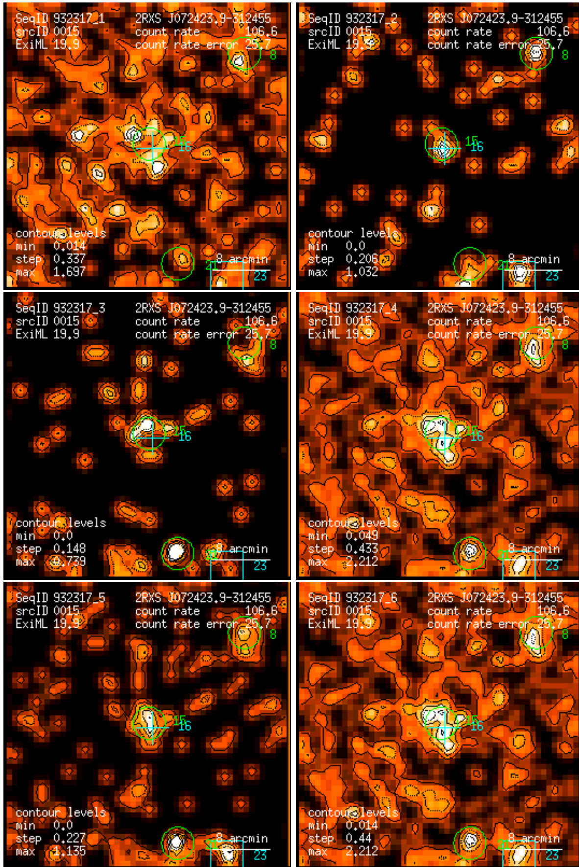
Figure 15: RASS 932317: detection 0015: band rate images, Gaussian filter: (1) PSPC channels 11 – 41, (2) 52 – 90, (3) 91 – 201, (4) 11 – 235, (5) 52 – 201, (6) 11 – 201. Broad band rates in counts/ks. Band rate contour levels in counts/ks/arcmin 2 .
