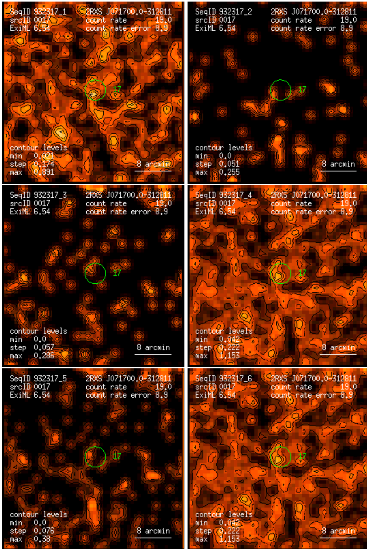
Figure 17: RASS 932317: detection 0017: band rate images, Gaussian filter: (1) PSPC channels 11 – 41, (2) 52 – 90, (3) 91 – 201, (4) 11 – 235, (5) 52 – 201, (6) 11 – 201. Broad band rates in counts/ks. Band rate contour levels in counts/ks/arcmin 2 .
