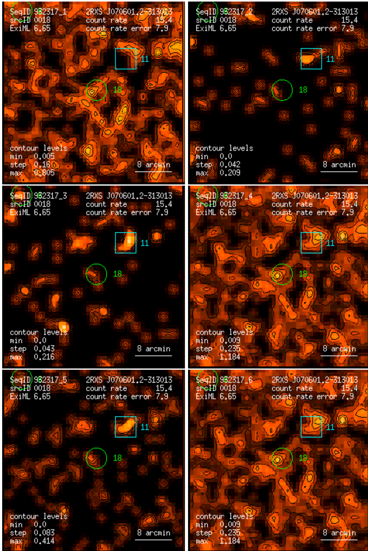
Figure 18: RASS 932317: detection 0018: band rate images, Gaussian filter: (1) PSPC channels 11 – 41, (2) 52 – 90, (3) 91 – 201, (4) 11 – 235, (5) 52 – 201, (6) 11 – 201. Broad band rates in counts/ks. Band rate contour levels in counts/ks/arcmin 2 .
