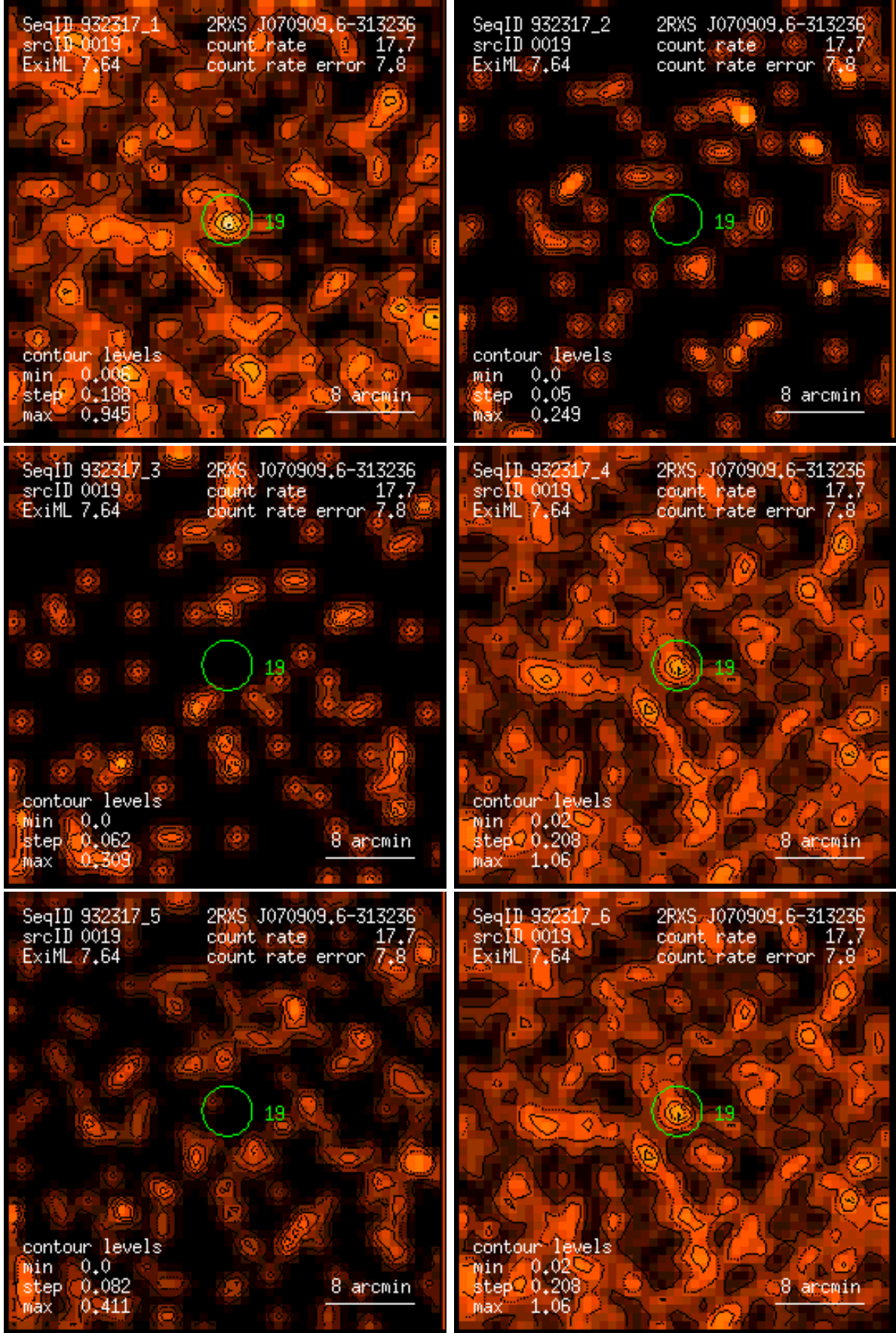
Figure 19: RASS 932317: detection 0019: band rate images, Gaussian filter: (1) PSPC channels 11 – 41, (2) 52 – 90, (3) 91 – 201, (4) 11 – 235, (5) 52 – 201, (6) 11 – 201. Broad band rates in counts/ks. Band rate contour levels in counts/ks/arcmin 2 .
