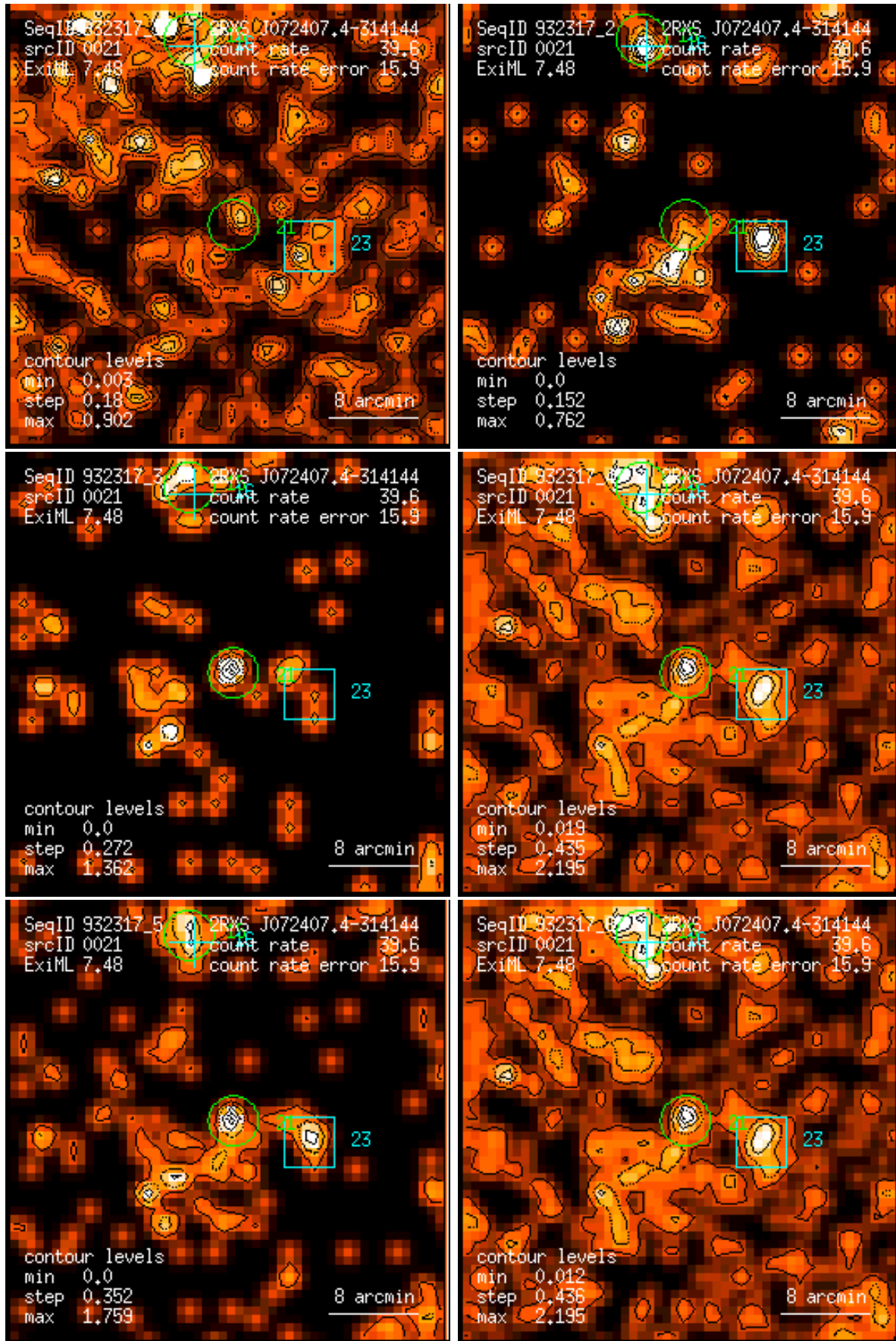
Figure 21: RASS 932317: detection 0021: band rate images, Gaussian filter: (1) PSPC channels 11 – 41, (2) 52 – 90, (3) 91 – 201, (4) 11 – 235, (5) 52 – 201, (6) 11 – 201. Broad band rates in counts/ks. Band rate contour levels in counts/ks/arcmin 2 .
