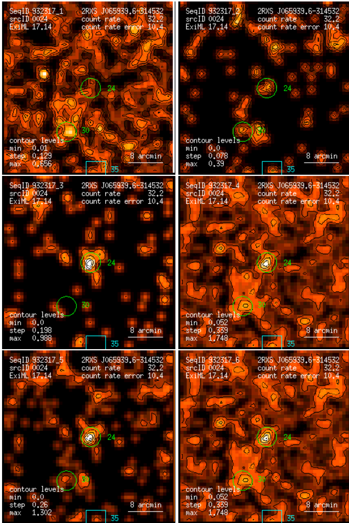
Figure 24: RASS 932317: detection 0024: band rate images, Gaussian filter: (1) PSPC channels 11 – 41, (2) 52 – 90, (3) 91 – 201, (4) 11 – 235, (5) 52 – 201, (6) 11 – 201. Broad band rates in counts/ks. Band rate contour levels in counts/ks/arcmin 2 .
