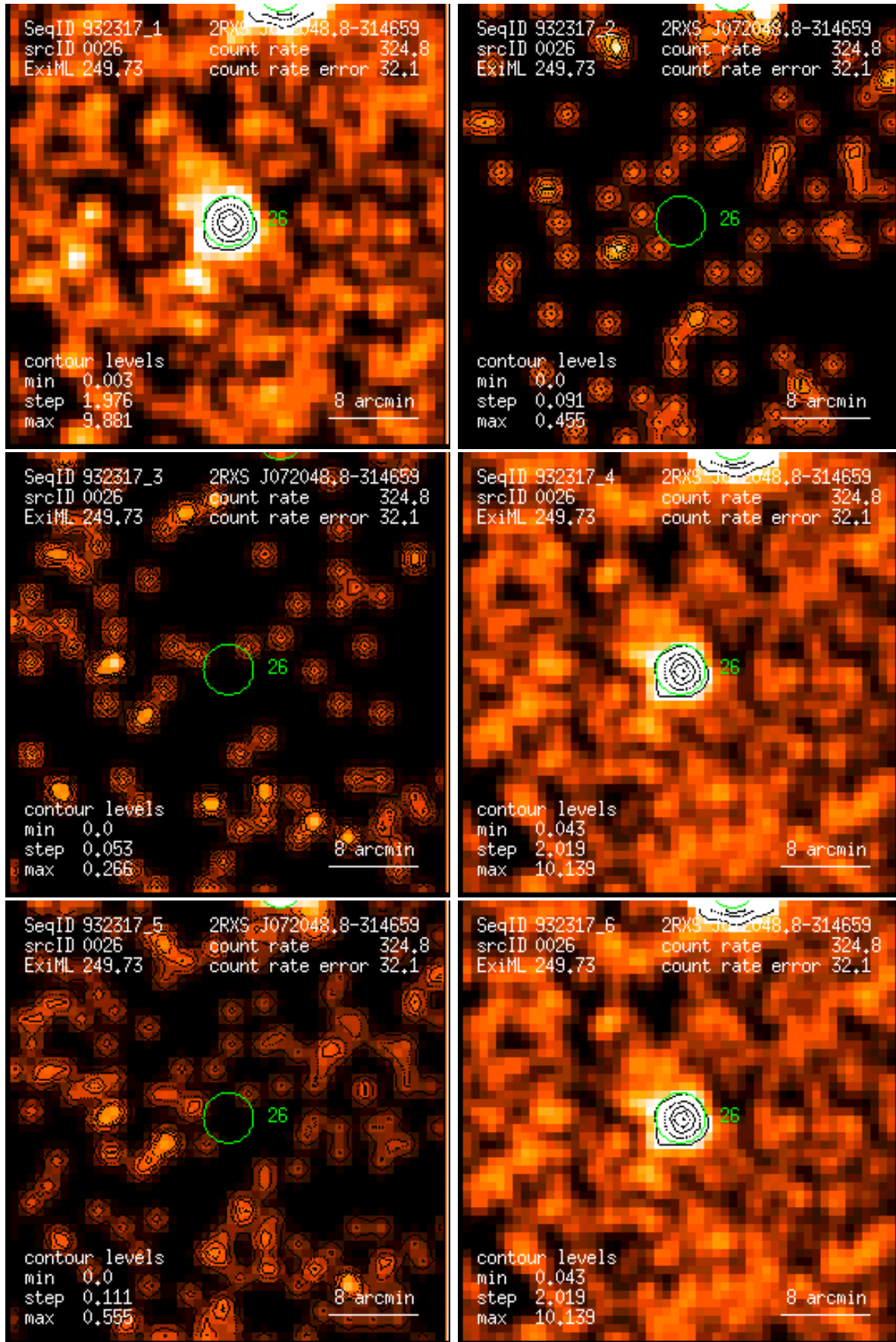
Figure 26: RASS 932317: detection 0026: band rate images, Gaussian filter: (1) PSPC channels 11 – 41, (2) 52 – 90, (3) 91 – 201, (4) 11 – 235, (5) 52 – 201, (6) 11 – 201. Broad band rates in counts/ks. Band rate contour levels in counts/ks/arcmin 2 .
