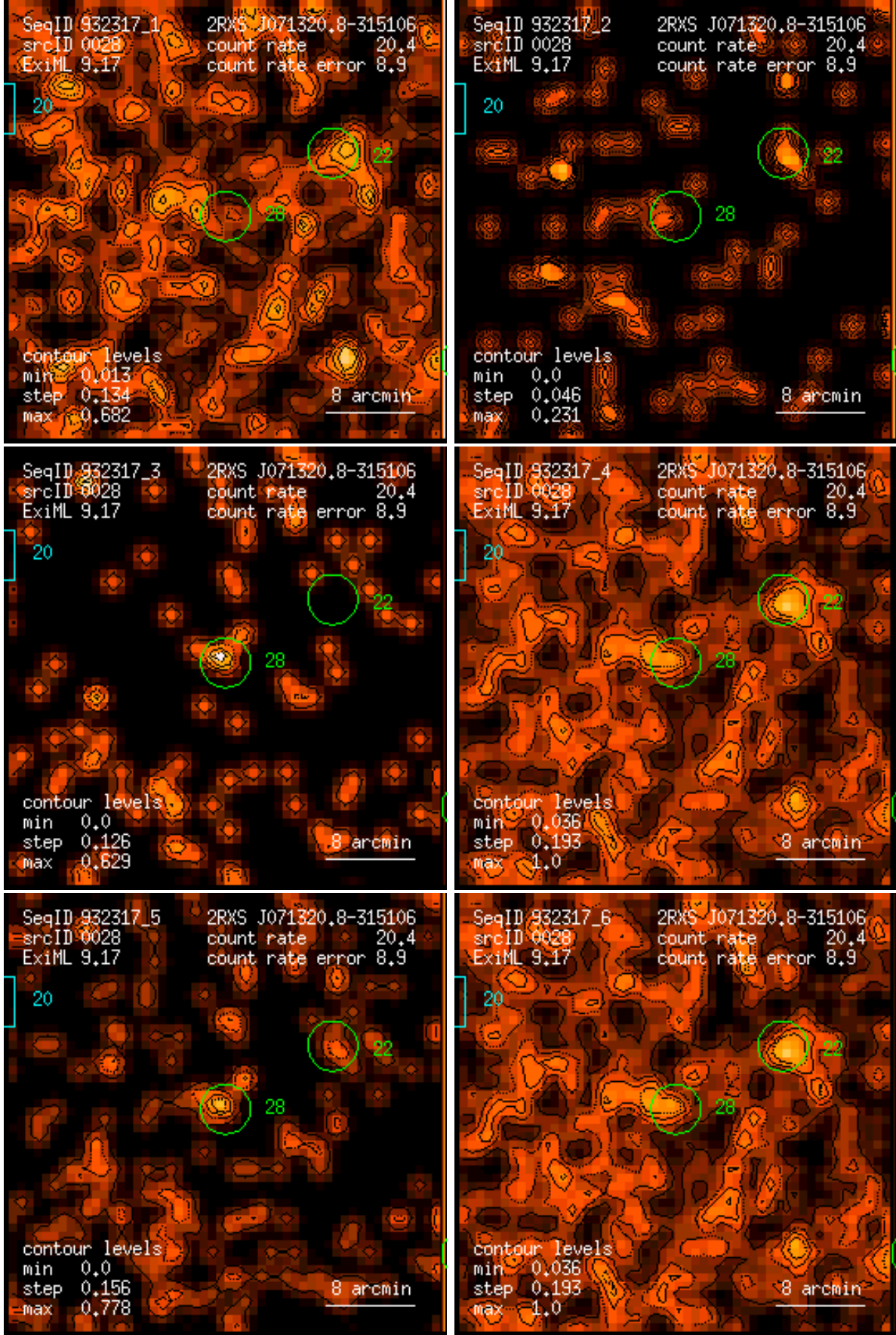
Figure 28: RASS 932317: detection 0028: band rate images, Gaussian filter: (1) PSPC channels 11 – 41, (2) 52 – 90, (3) 91 – 201, (4) 11 – 235, (5) 52 – 201, (6) 11 – 201. Broad band rates in counts/ks. Band rate contour levels in counts/ks/arcmin 2 .
