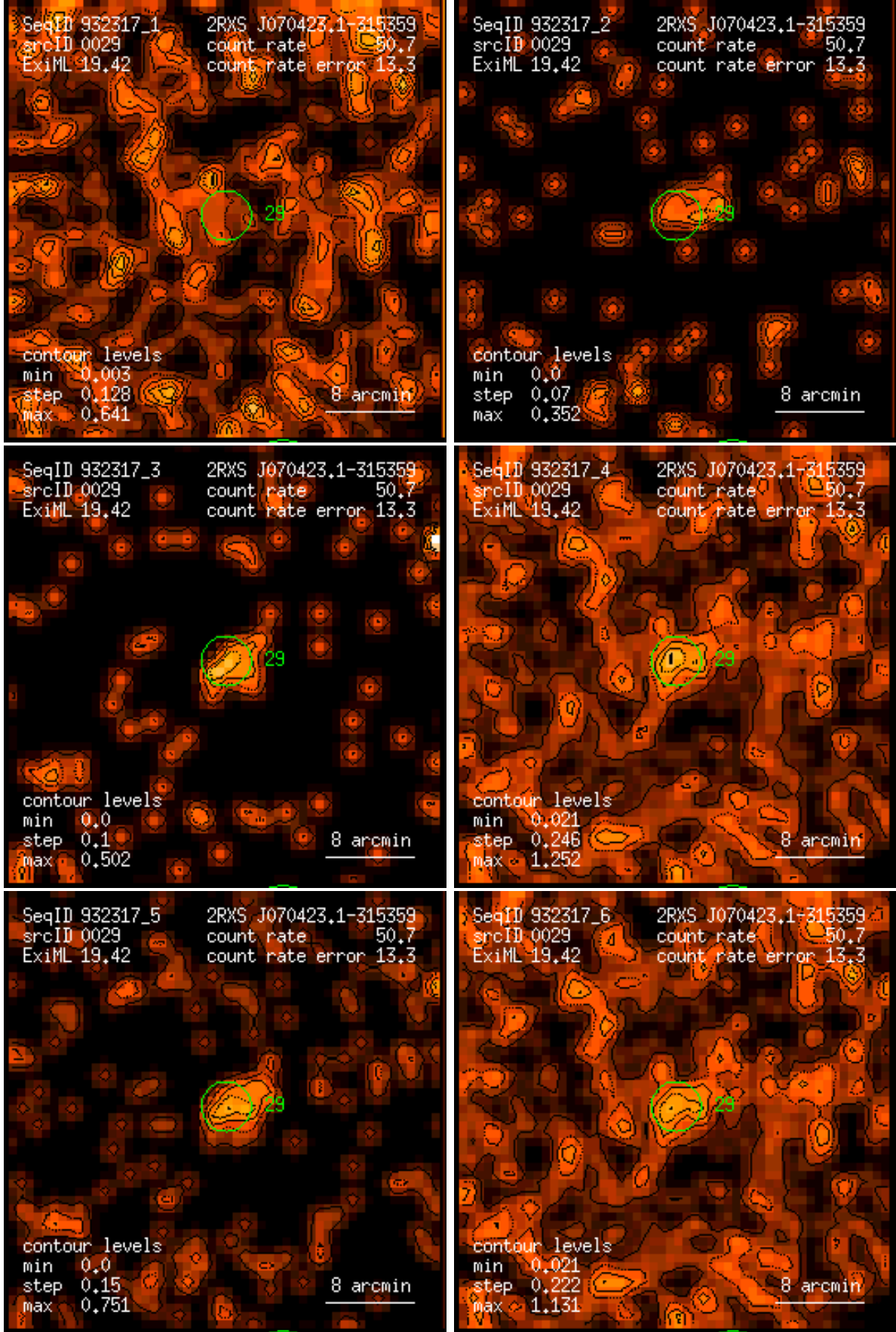
Figure 29: RASS 932317: detection 0029: band rate images, Gaussian filter: (1) PSPC channels 11 – 41, (2) 52 – 90, (3) 91 – 201, (4) 11 – 235, (5) 52 – 201, (6) 11 – 201. Broad band rates in counts/ks. Band rate contour levels in counts/ks/arcmin 2 .
