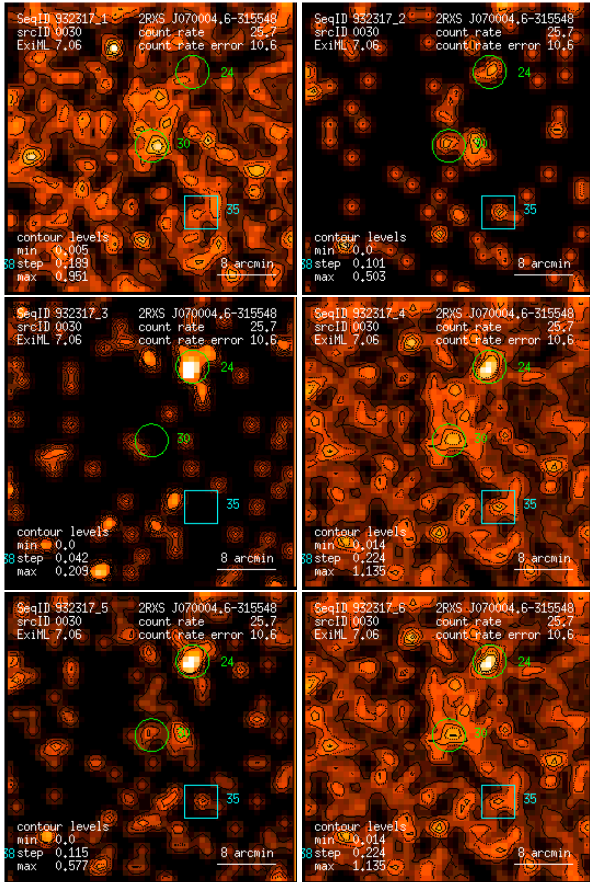
Figure 30: RASS 932317: detection 0030: band rate images, Gaussian filter: (1) PSPC channels 11 – 41, (2) 52 – 90, (3) 91 – 201, (4) 11 – 235, (5) 52 – 201, (6) 11 – 201. Broad band rates in counts/ks. Band rate contour levels in counts/ks/arcmin 2 .
