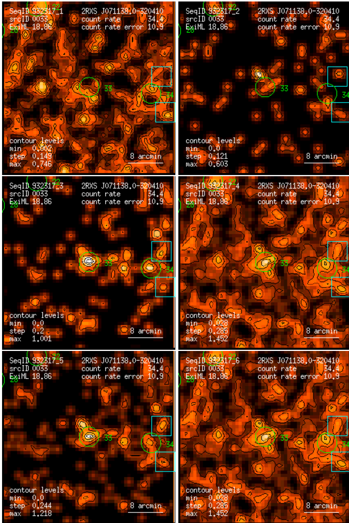
Figure 33: RASS 932317: detection 0033: band rate images, Gaussian filter: (1) PSPC channels 11 – 41, (2) 52 – 90, (3) 91 – 201, (4) 11 – 235, (5) 52 – 201, (6) 11 – 201. Broad band rates in counts/ks. Band rate contour levels in counts/ks/arcmin 2 .
