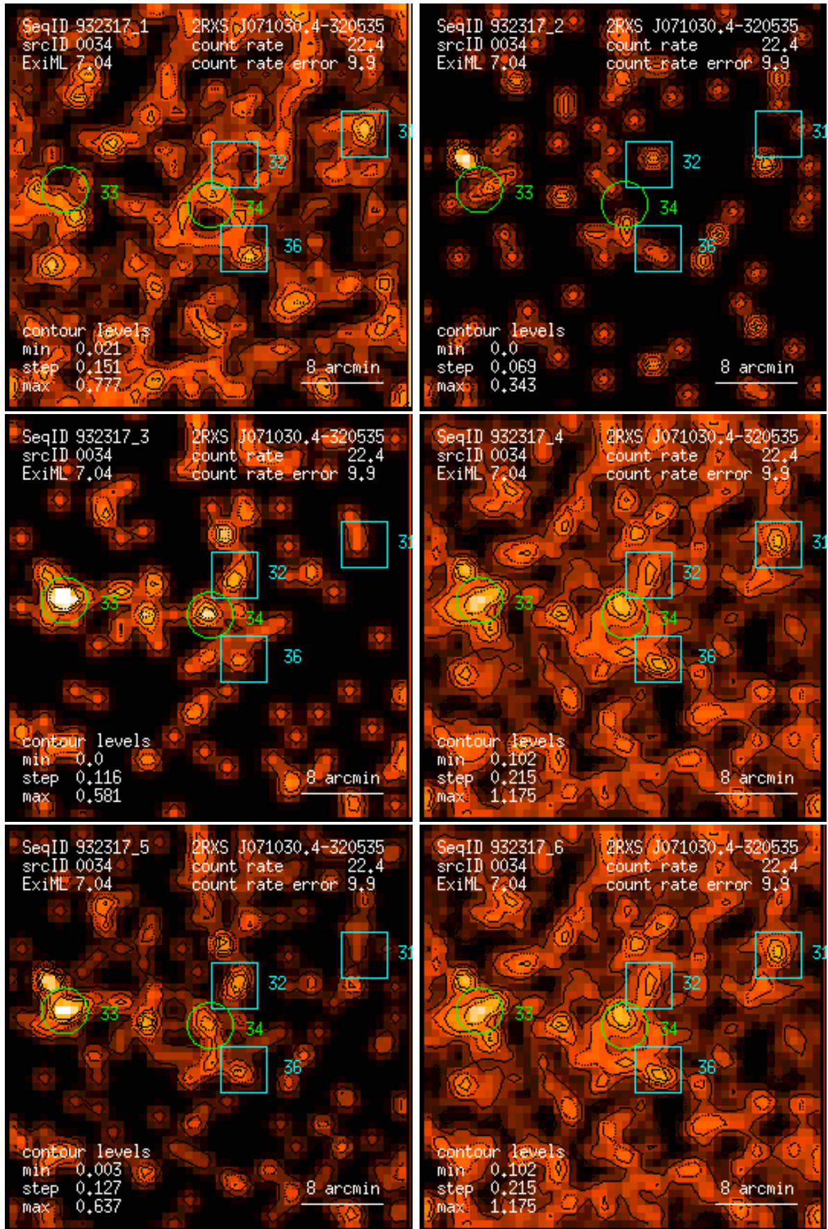
Figure 34: RASS 932317: detection 0034: band rate images, Gaussian filter: (1) PSPC channels 11 – 41, (2) 52 – 90, (3) 91 – 201, (4) 11 – 235, (5) 52 – 201, (6) 11 – 201. Broad band rates in counts/ks. Band rate contour levels in counts/ks/arcmin 2 .
