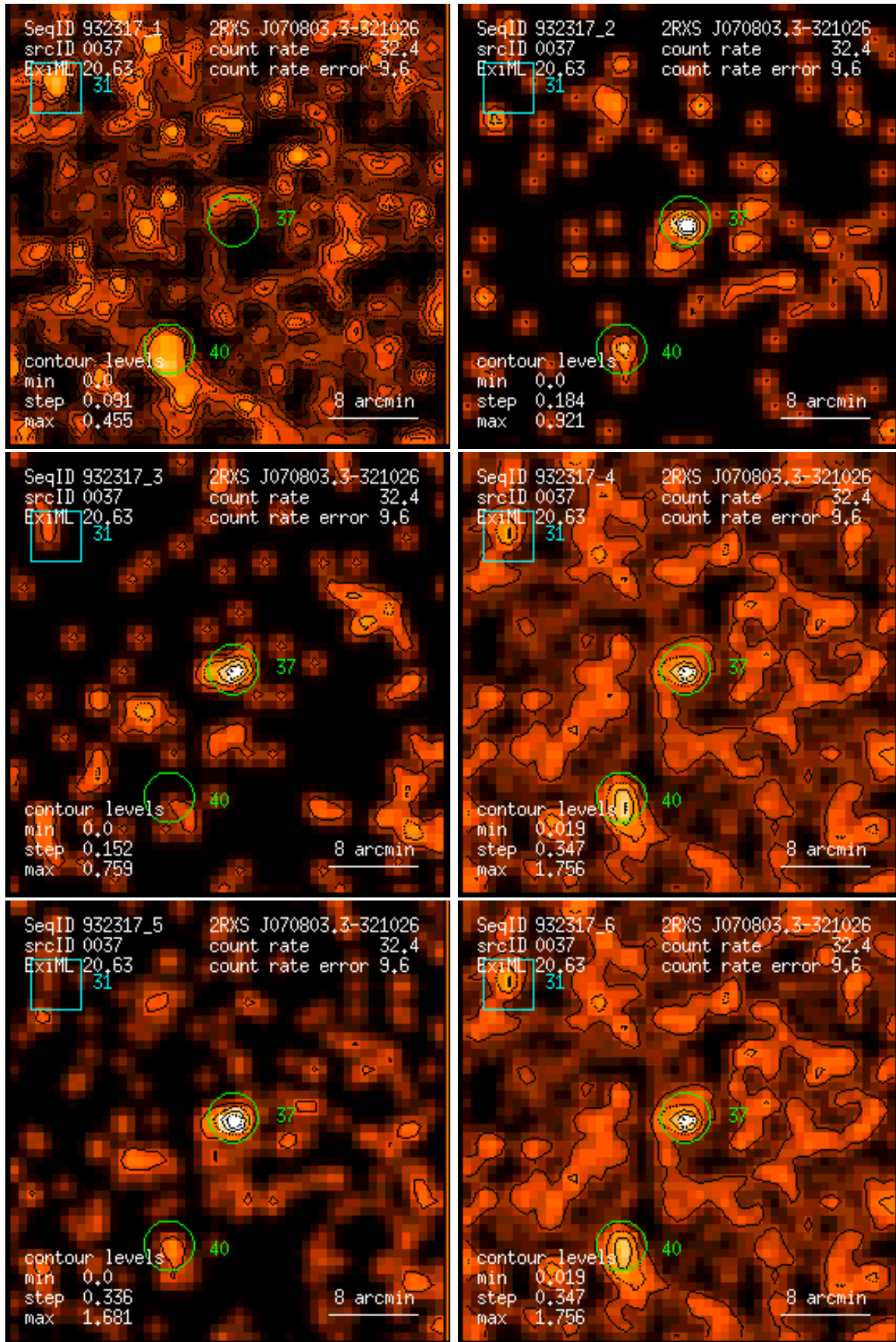
Figure 37: RASS 932317: detection 0037: band rate images, Gaussian filter: (1) PSPC channels 11 – 41, (2) 52 – 90, (3) 91 – 201, (4) 11 – 235, (5) 52 – 201, (6) 11 – 201. Broad band rates in counts/ks. Band rate contour levels in counts/ks/arcmin 2 .
