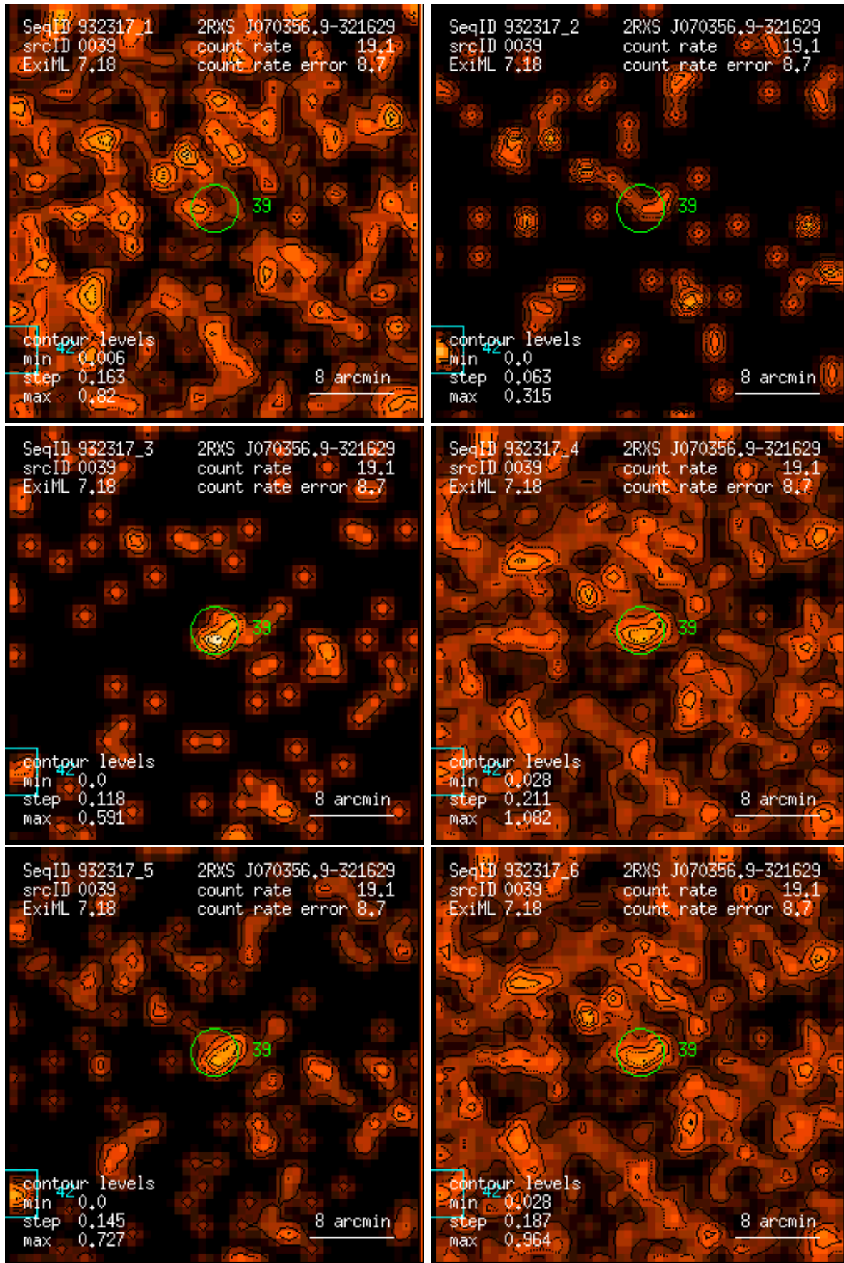
Figure 39: RASS 932317: detection 0039: band rate images, Gaussian filter: (1) PSPC channels 11 – 41, (2) 52 – 90, (3) 91 – 201, (4) 11 – 235, (5) 52 – 201, (6) 11 – 201. Broad band rates in counts/ks. Band rate contour levels in counts/ks/arcmin 2 .
