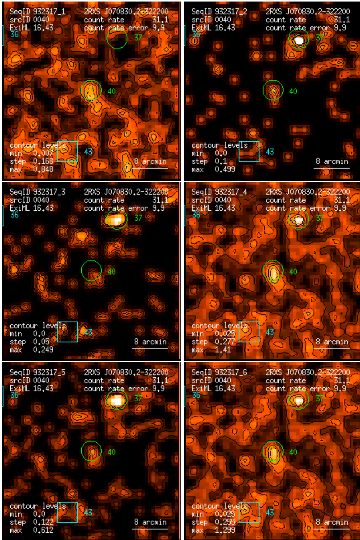
Figure 40: RASS 932317: detection 0040: band rate images, Gaussian filter: (1) PSPC channels 11 – 41, (2) 52 – 90, (3) 91 – 201, (4) 11 – 235, (5) 52 – 201, (6) 11 – 201. Broad band rates in counts/ks. Band rate contour levels in counts/ks/arcmin 2 .
