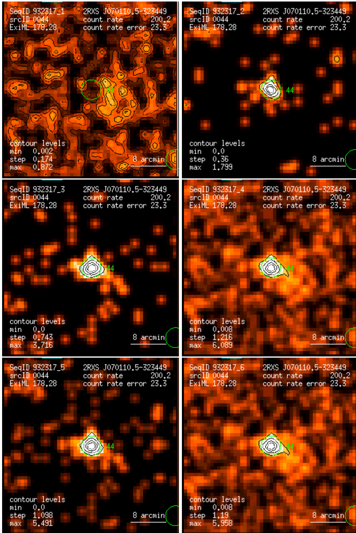
Figure 44: RASS 932317: detection 0044: band rate images, Gaussian filter: (1) PSPC channels 11 – 41, (2) 52 – 90, (3) 91 – 201, (4) 11 – 235, (5) 52 – 201, (6) 11 – 201. Broad band rates in counts/ks. Band rate contour levels in counts/ks/arcmin 2 .
