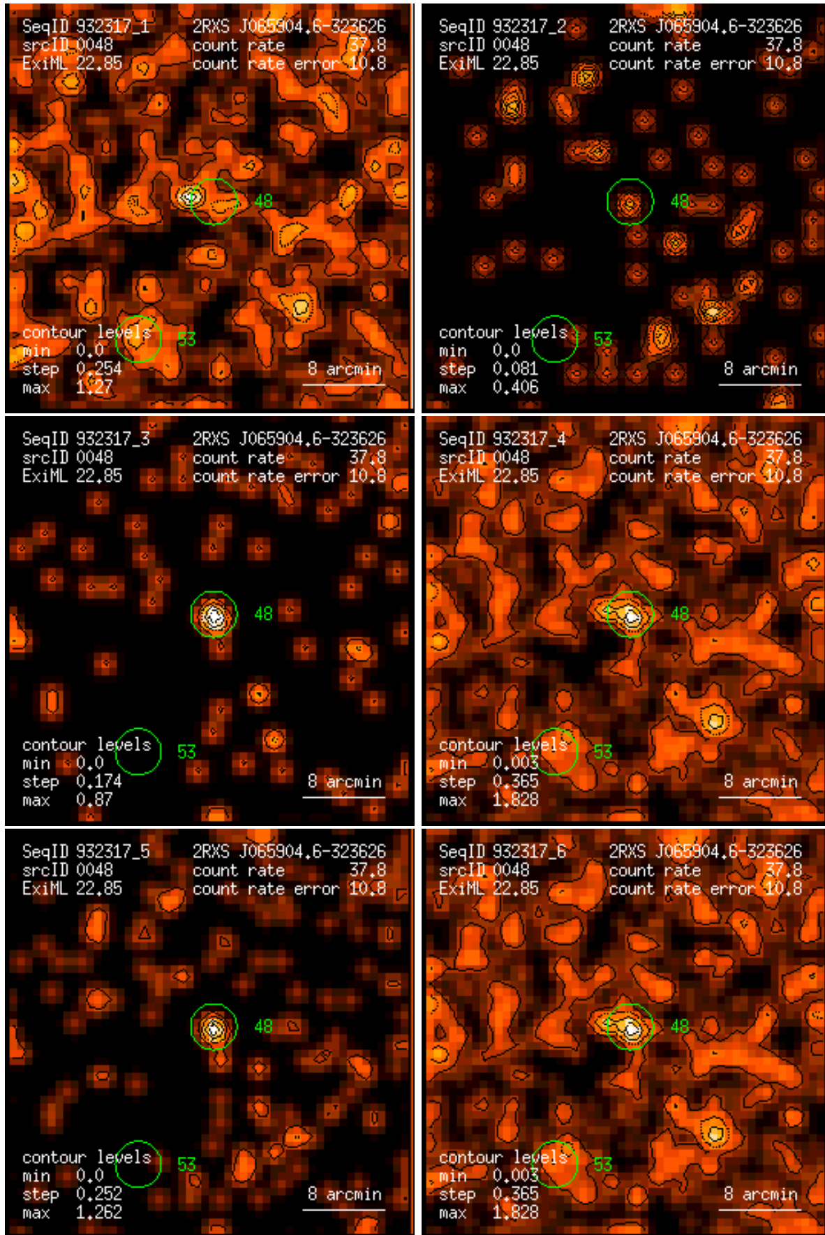
Figure 48: RASS 932317: detection 0048: band rate images, Gaussian filter: (1) PSPC channels 11 – 41, (2) 52 – 90, (3) 91 – 201, (4) 11 – 235, (5) 52 – 201, (6) 11 – 201. Broad band rates in counts/ks. Band rate contour levels in counts/ks/arcmin 2 .
