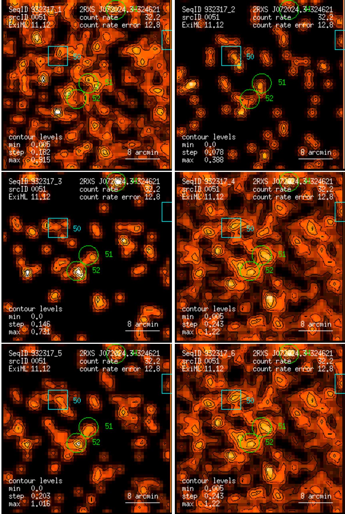
Figure 51: RASS 932317: detection 0051: band rate images, Gaussian filter: (1) PSPC channels 11 – 41, (2) 52 – 90, (3) 91 – 201, (4) 11 – 235, (5) 52 – 201, (6) 11 – 201. Broad band rates in counts/ks. Band rate contour levels in counts/ks/arcmin 2 .
