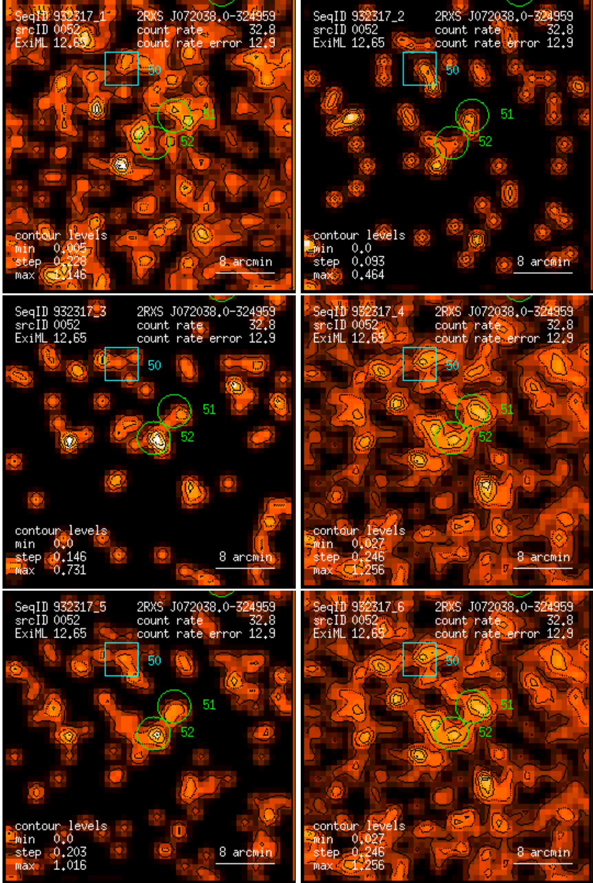
Figure 52: RASS 932317: detection 0052: band rate images, Gaussian filter: (1) PSPC channels 11 – 41, (2) 52 – 90, (3) 91 – 201, (4) 11 – 235, (5) 52 – 201, (6) 11 – 201. Broad band rates in counts/ks. Band rate contour levels in counts/ks/arcmin 2 .
