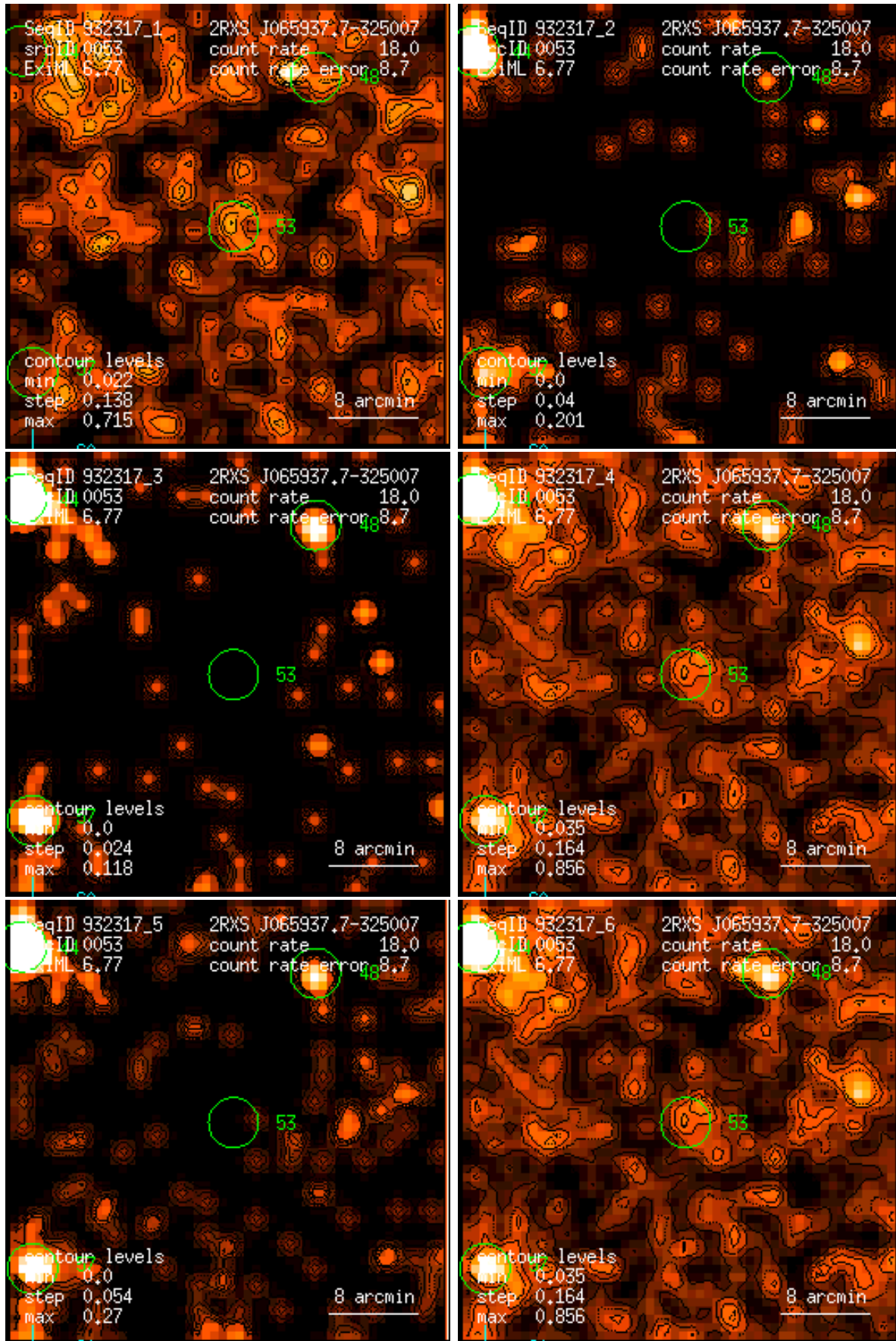
Figure 53: RASS 932317: detection 0053: band rate images, Gaussian filter: (1) PSPC channels 11 – 41, (2) 52 – 90, (3) 91 – 201, (4) 11 – 235, (5) 52 – 201, (6) 11 – 201. Broad band rates in counts/ks. Band rate contour levels in counts/ks/arcmin 2 .
