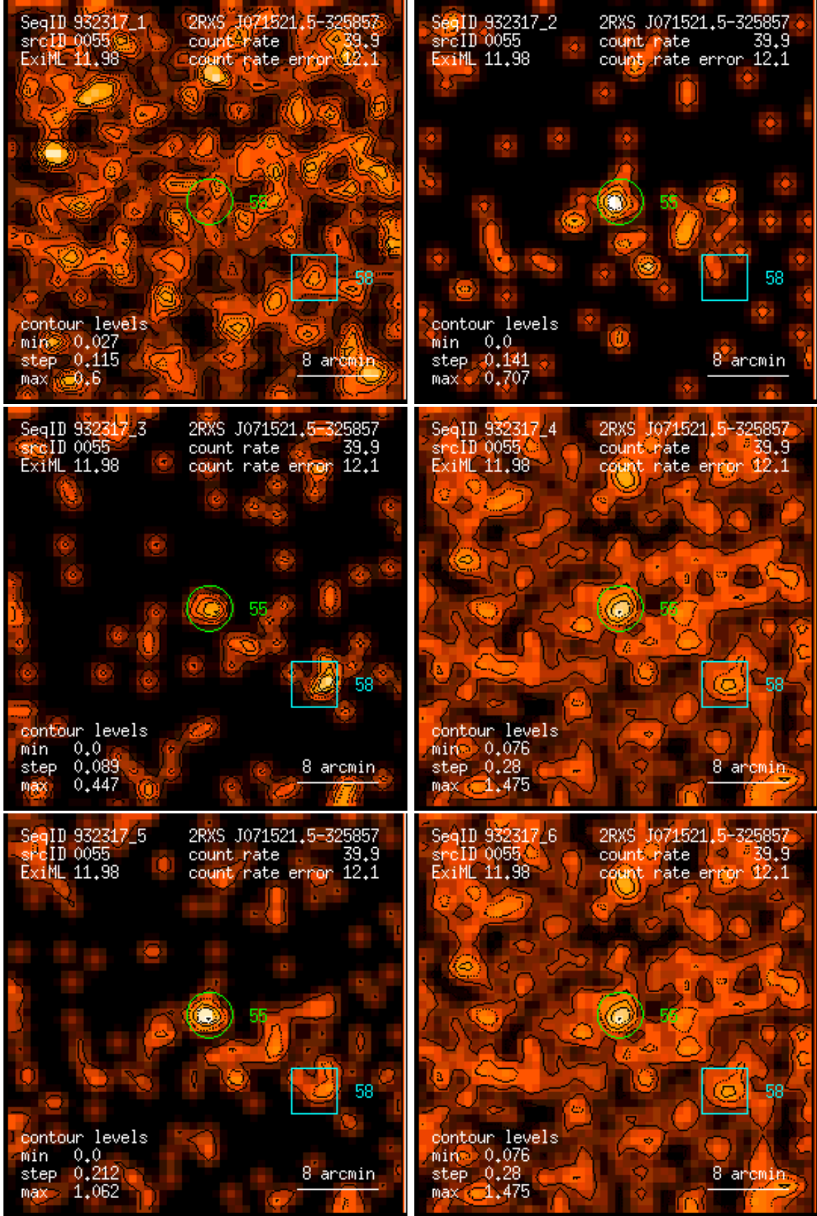
Figure 55: RASS 932317: detection 0055: band rate images, Gaussian filter: (1) PSPC channels 11 – 41, (2) 52 – 90, (3) 91 – 201, (4) 11 – 235, (5) 52 – 201, (6) 11 – 201. Broad band rates in counts/ks. Band rate contour levels in counts/ks/arcmin 2 .
