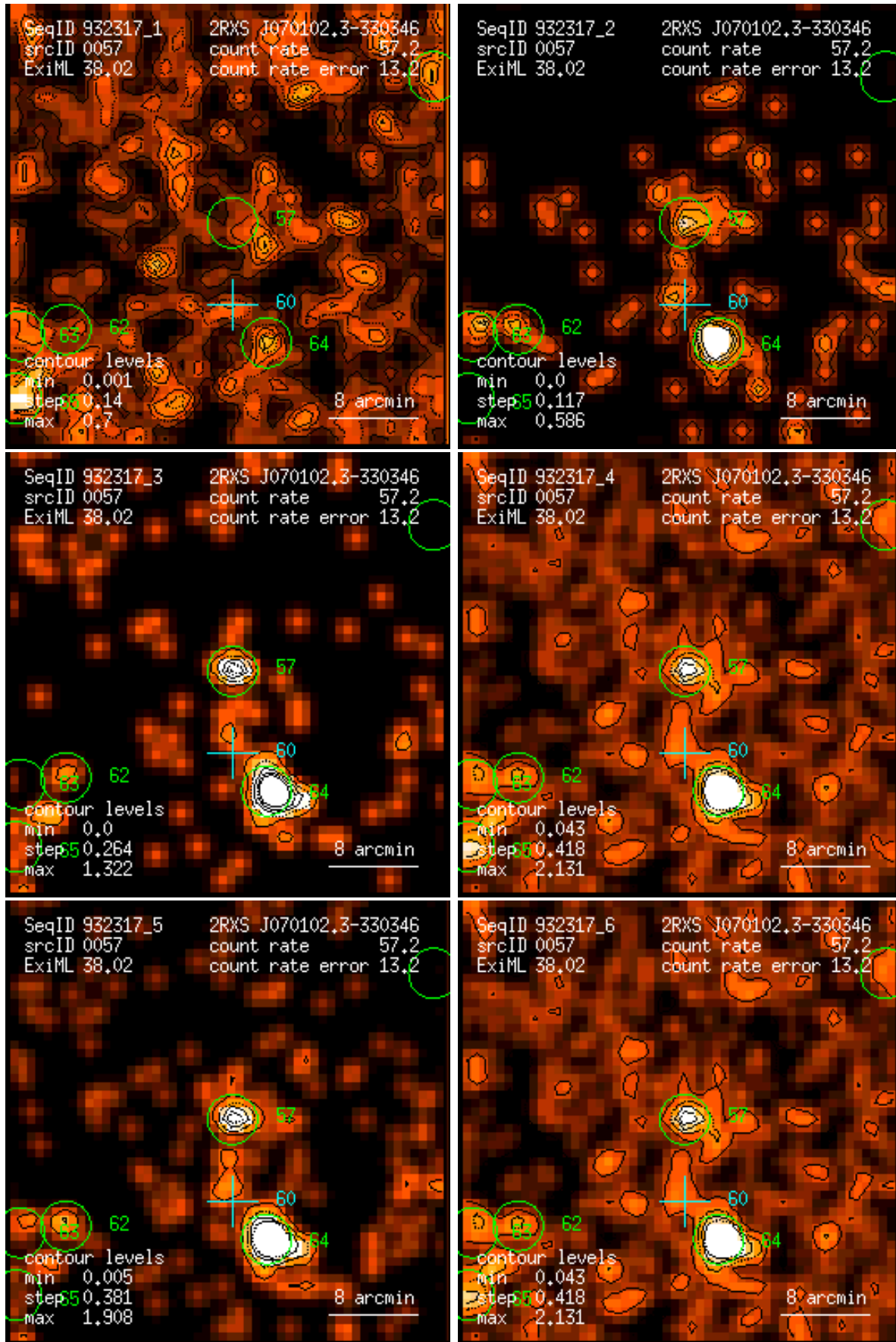
Figure 57: RASS 932317: detection 0057: band rate images, Gaussian filter: (1) PSPC channels 11 – 41, (2) 52 – 90, (3) 91 – 201, (4) 11 – 235, (5) 52 – 201, (6) 11 – 201. Broad band rates in counts/ks. Band rate contour levels in counts/ks/arcmin 2 .
