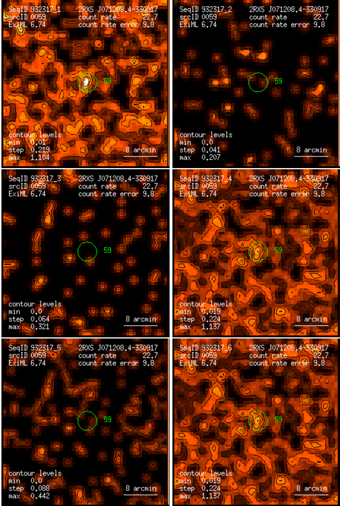
Figure 59: RASS 932317: detection 0059: band rate images, Gaussian filter: (1) PSPC channels 11 – 41, (2) 52 – 90, (3) 91 – 201, (4) 11 – 235, (5) 52 – 201, (6) 11 – 201. Broad band rates in counts/ks. Band rate contour levels in counts/ks/arcmin 2 .
