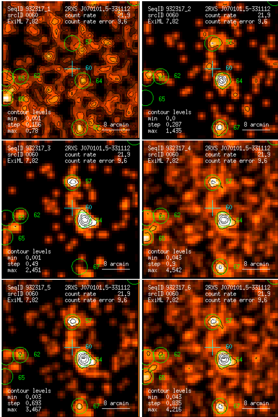
Figure 60: RASS 932317: detection 0060: band rate images, Gaussian filter: (1) PSPC channels 11 – 41, (2) 52 – 90, (3) 91 – 201, (4) 11 – 235, (5) 52 – 201, (6) 11 – 201. Broad band rates in counts/ks. Band rate contour levels in counts/ks/arcmin 2 .
