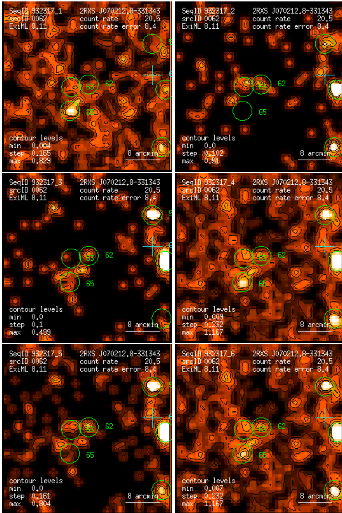
Figure 62: RASS 932317: detection 0062: band rate images, Gaussian filter: (1) PSPC channels 11 – 41, (2) 52 – 90, (3) 91 – 201, (4) 11 – 235, (5) 52 – 201, (6) 11 – 201. Broad band rates in counts/ks. Band rate contour levels in counts/ks/arcmin 2 .
