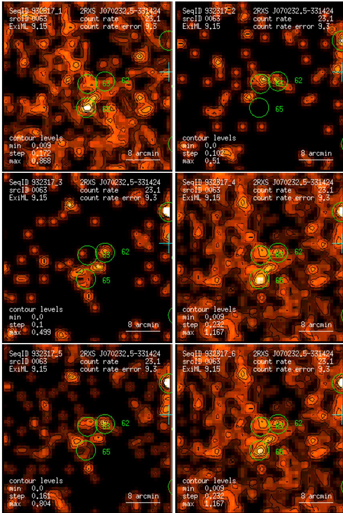
Figure 63: RASS 932317: detection 0063: band rate images, Gaussian filter: (1) PSPC channels 11 – 41, (2) 52 – 90, (3) 91 – 201, (4) 11 – 235, (5) 52 – 201, (6) 11 – 201. Broad band rates in counts/ks. Band rate contour levels in counts/ks/arcmin 2 .
