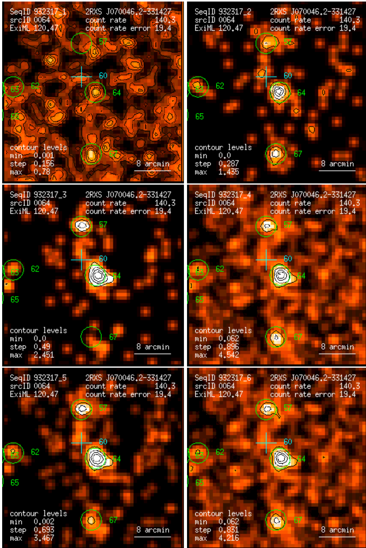
Figure 64: RASS 932317: detection 0064: band rate images, Gaussian filter: (1) PSPC channels 11 – 41, (2) 52 – 90, (3) 91 – 201, (4) 11 – 235, (5) 52 – 201, (6) 11 – 201. Broad band rates in counts/ks. Band rate contour levels in counts/ks/arcmin 2 .
