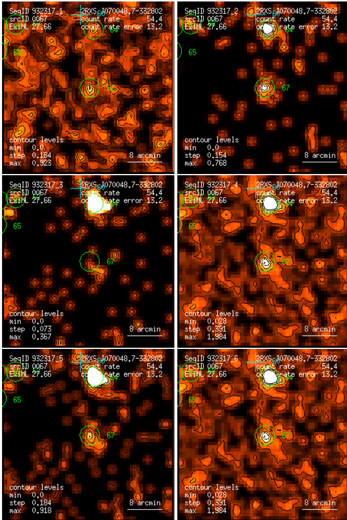
Figure 67: RASS 932317: detection 0067: band rate images, Gaussian filter: (1) PSPC channels 11 – 41, (2) 52 – 90, (3) 91 – 201, (4) 11 – 235, (5) 52 – 201, (6) 11 – 201. Broad band rates in counts/ks. Band rate contour levels in counts/ks/arcmin 2 .
