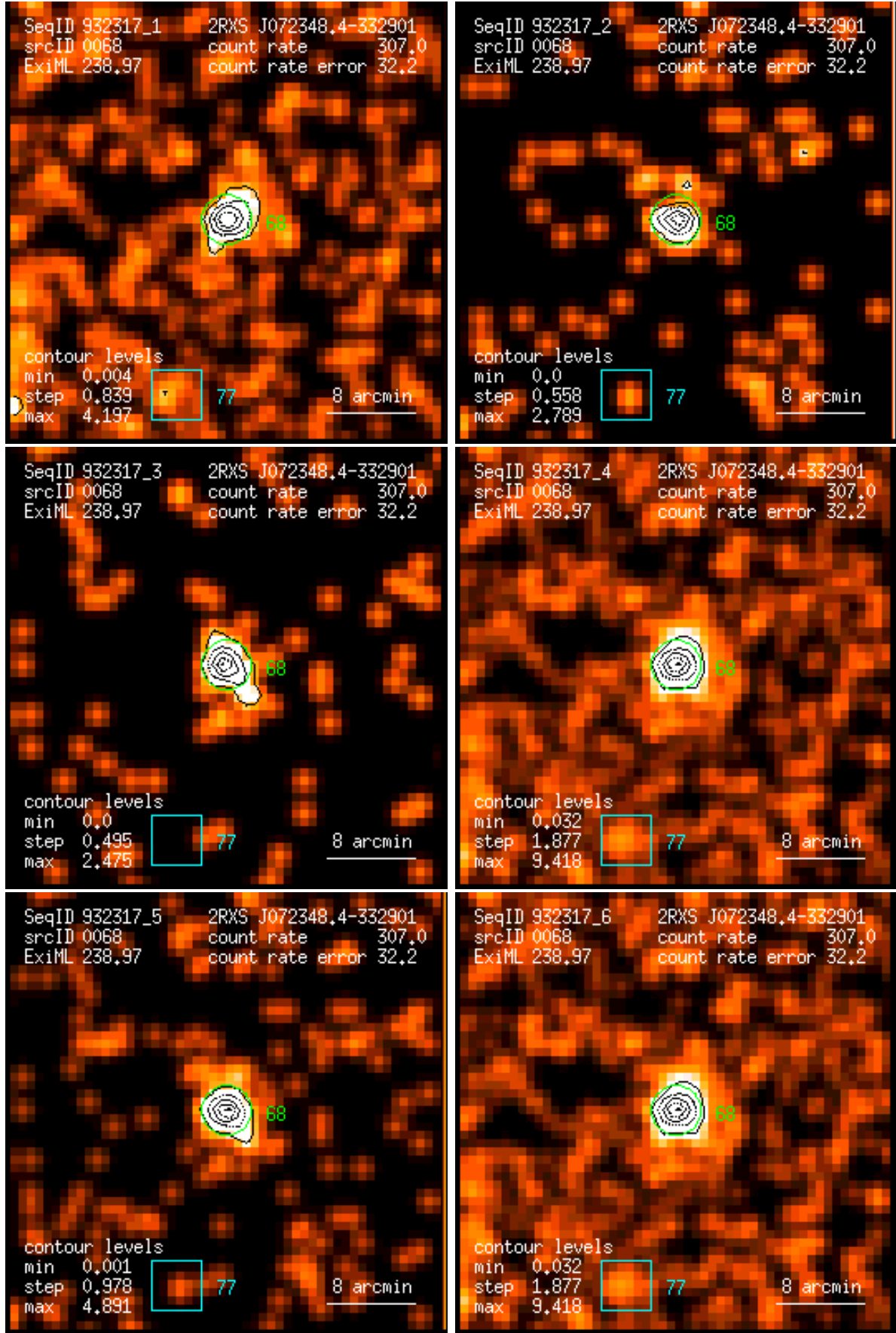
Figure 68: RASS 932317: detection 0068: band rate images, Gaussian filter: (1) PSPC channels 11 – 41, (2) 52 – 90, (3) 91 – 201, (4) 11 – 235, (5) 52 – 201, (6) 11 – 201. Broad band rates in counts/ks. Band rate contour levels in counts/ks/arcmin 2 .
