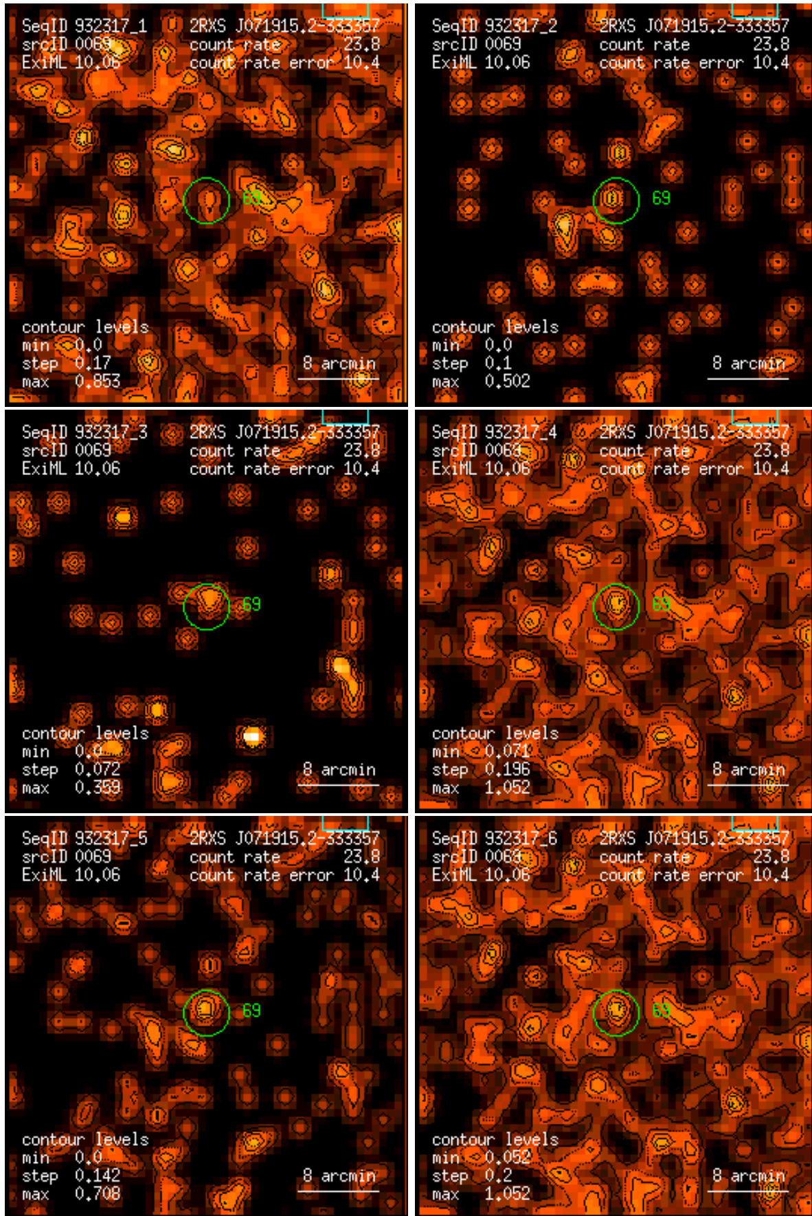
Figure 69: RASS 932317: detection 0069: band rate images, Gaussian filter: (1) PSPC channels 11 – 41, (2) 52 – 90, (3) 91 – 201, (4) 11 – 235, (5) 52 – 201, (6) 11 – 201. Broad band rates in counts/ks. Band rate contour levels in counts/ks/arcmin 2 .
