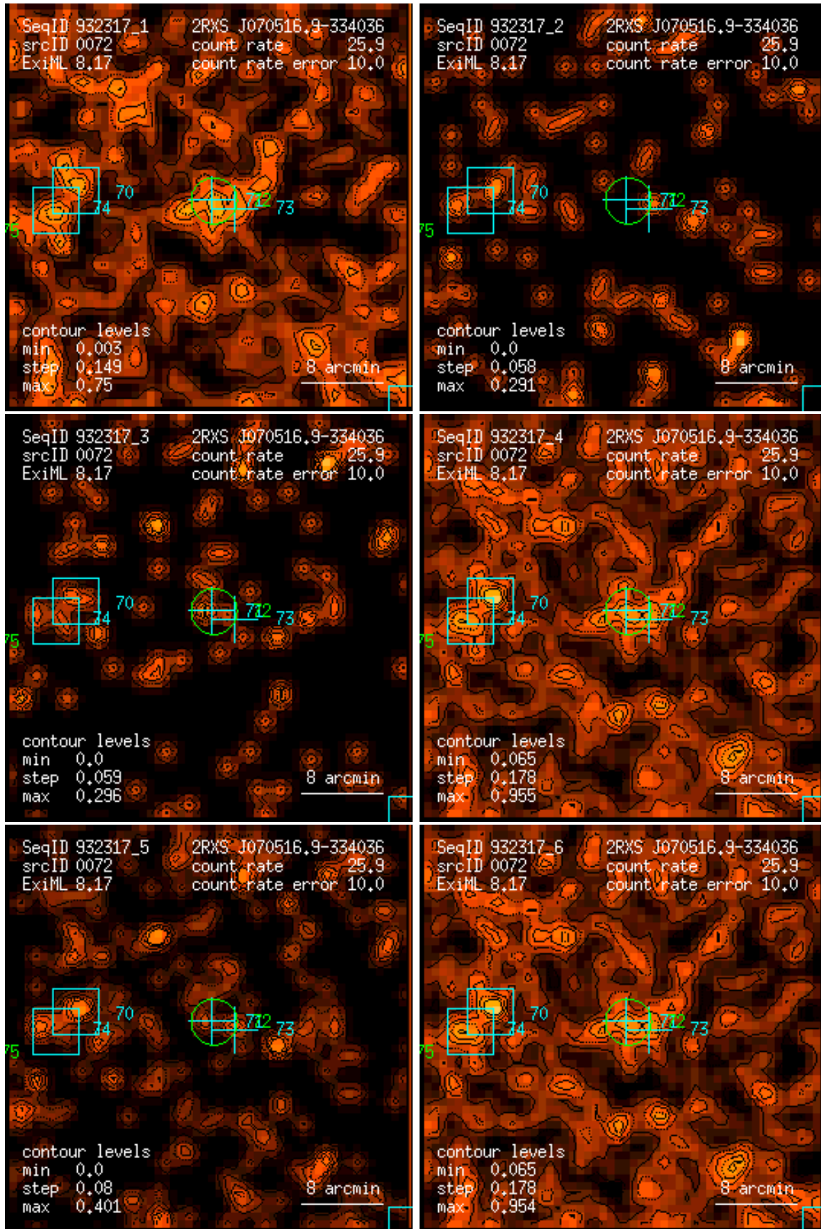
Figure 72: RASS 932317: detection 0072: band rate images, Gaussian filter: (1) PSPC channels 11 – 41, (2) 52 – 90, (3) 91 – 201, (4) 11 – 235, (5) 52 – 201, (6) 11 – 201. Broad band rates in counts/ks. Band rate contour levels in counts/ks/arcmin 2 .
