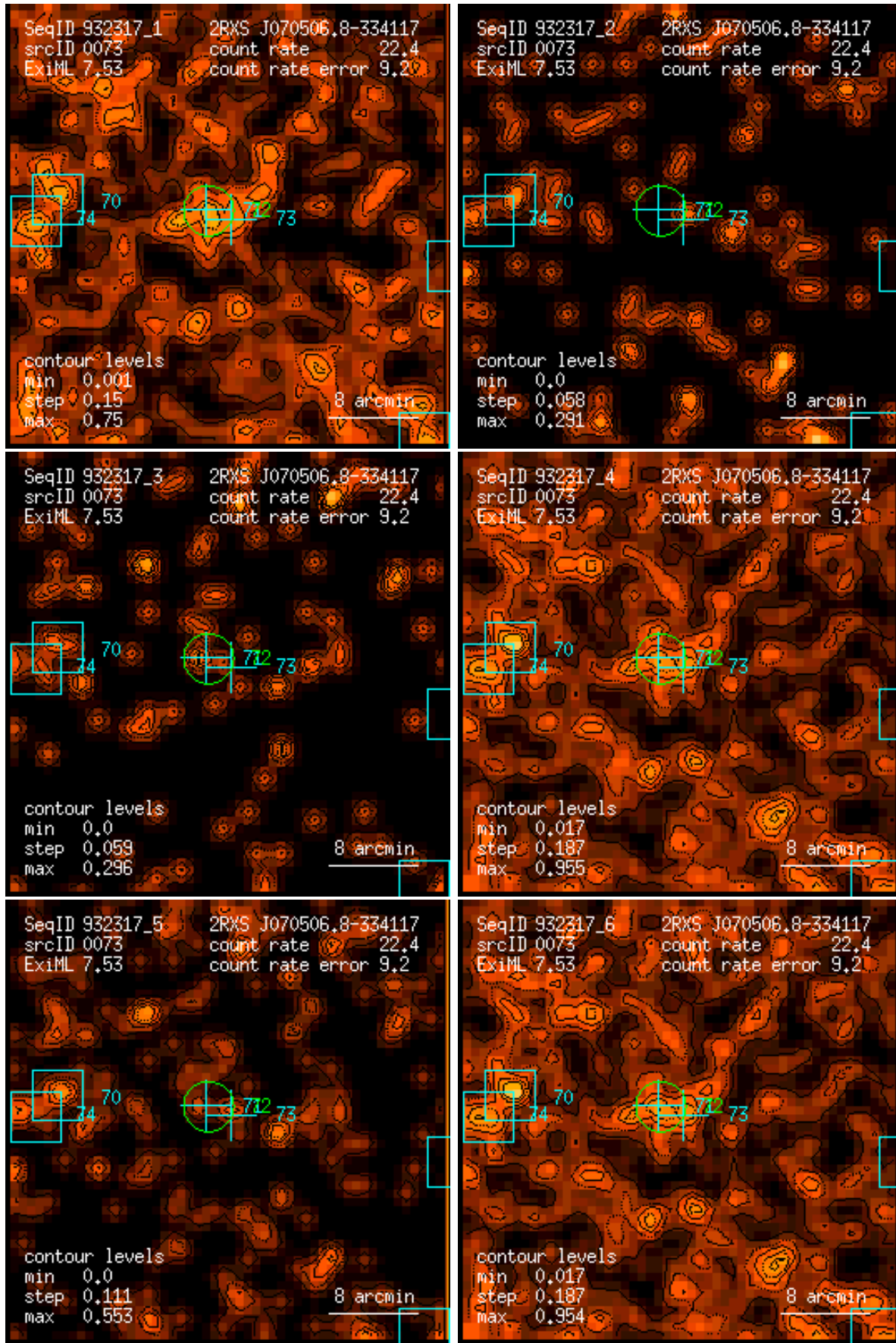
Figure 73: RASS 932317: detection 0073: band rate images, Gaussian filter: (1) PSPC channels 11 – 41, (2) 52 – 90, (3) 91 – 201, (4) 11 – 235, (5) 52 – 201, (6) 11 – 201. Broad band rates in counts/ks. Band rate contour levels in counts/ks/arcmin 2 .
