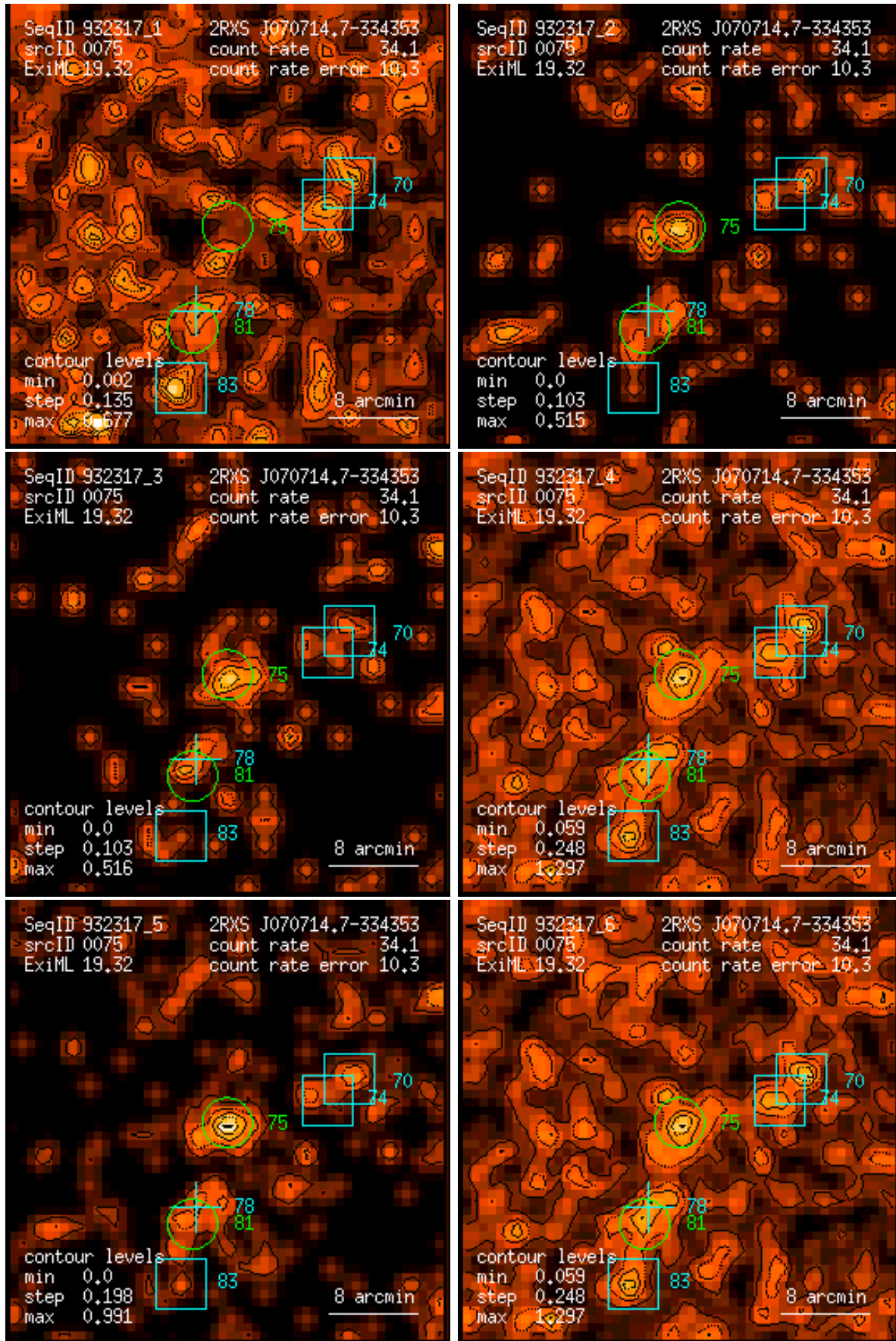
Figure 75: RASS 932317: detection 0075: band rate images, Gaussian filter: (1) PSPC channels 11 – 41, (2) 52 – 90, (3) 91 – 201, (4) 11 – 235, (5) 52 – 201, (6) 11 – 201. Broad band rates in counts/ks. Band rate contour levels in counts/ks/arcmin 2 .
