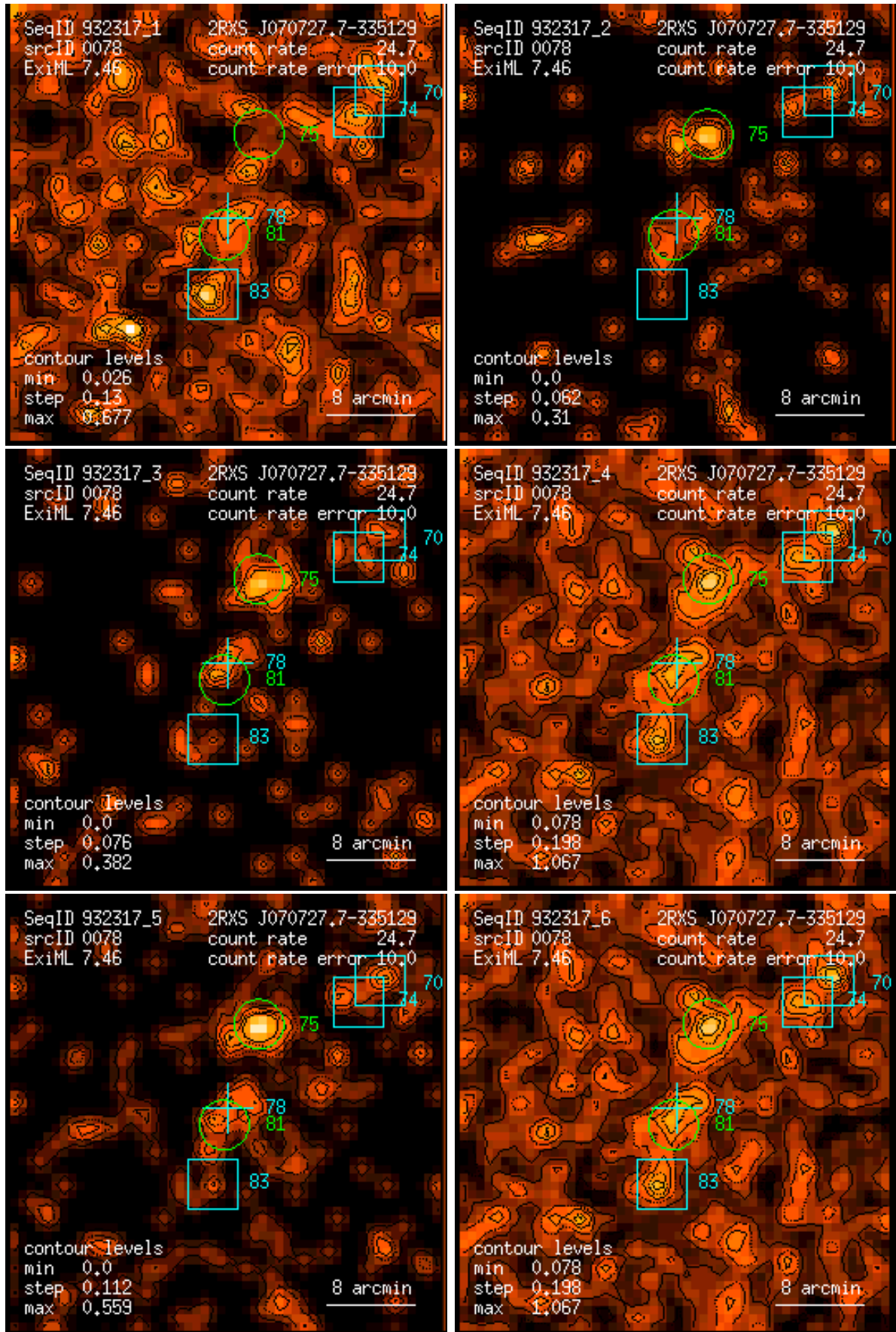
Figure 78: RASS 932317: detection 0078: band rate images, Gaussian filter: (1) PSPC channels 11 – 41, (2) 52 – 90, (3) 91 – 201, (4) 11 – 235, (5) 52 – 201, (6) 11 – 201. Broad band rates in counts/ks. Band rate contour levels in counts/ks/arcmin 2 .
