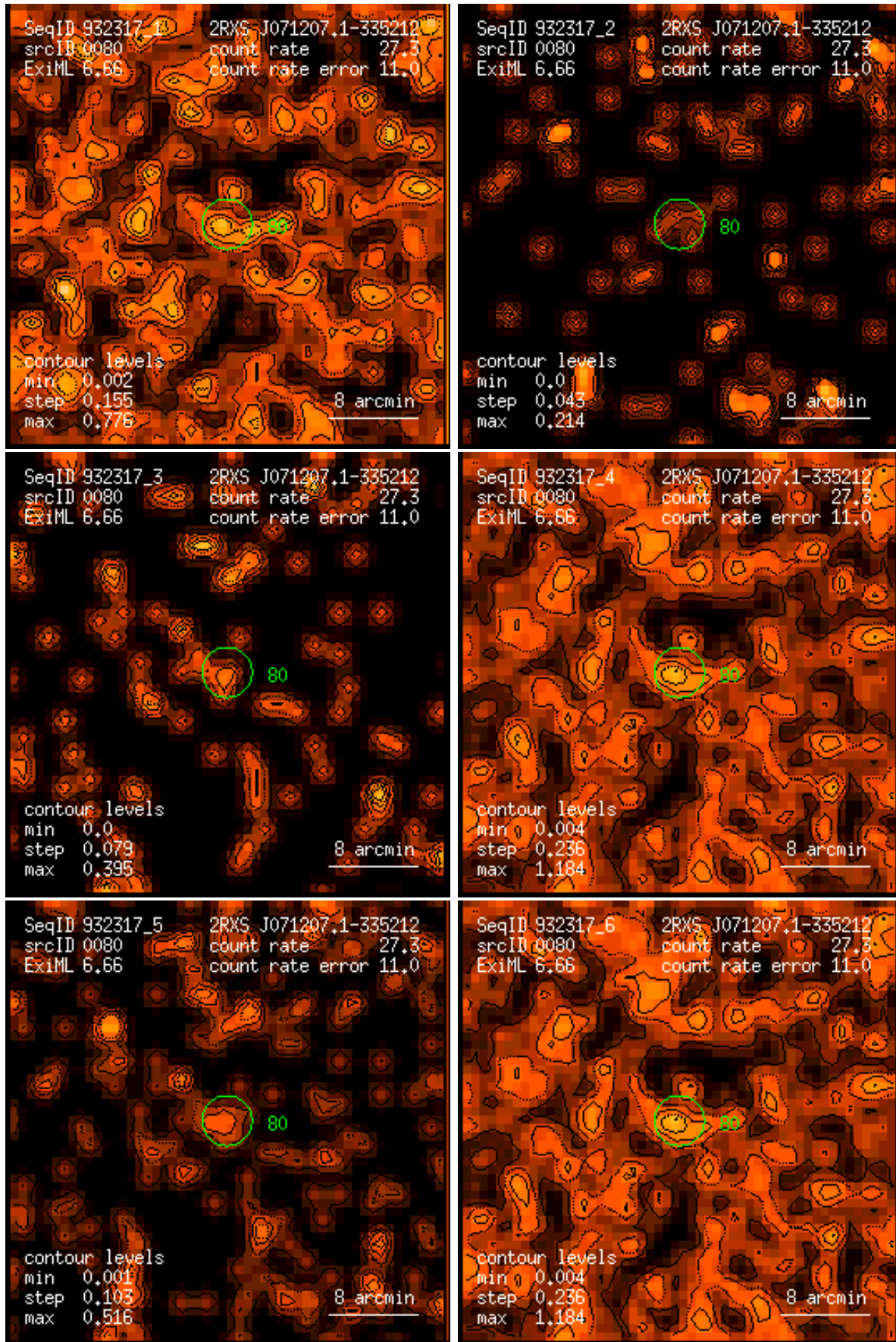
Figure 80: RASS 932317: detection 0080: band rate images, Gaussian filter: (1) PSPC channels 11 – 41, (2) 52 – 90, (3) 91 – 201, (4) 11 – 235, (5) 52 – 201, (6) 11 – 201. Broad band rates in counts/ks. Band rate contour levels in counts/ks/arcmin 2 .
