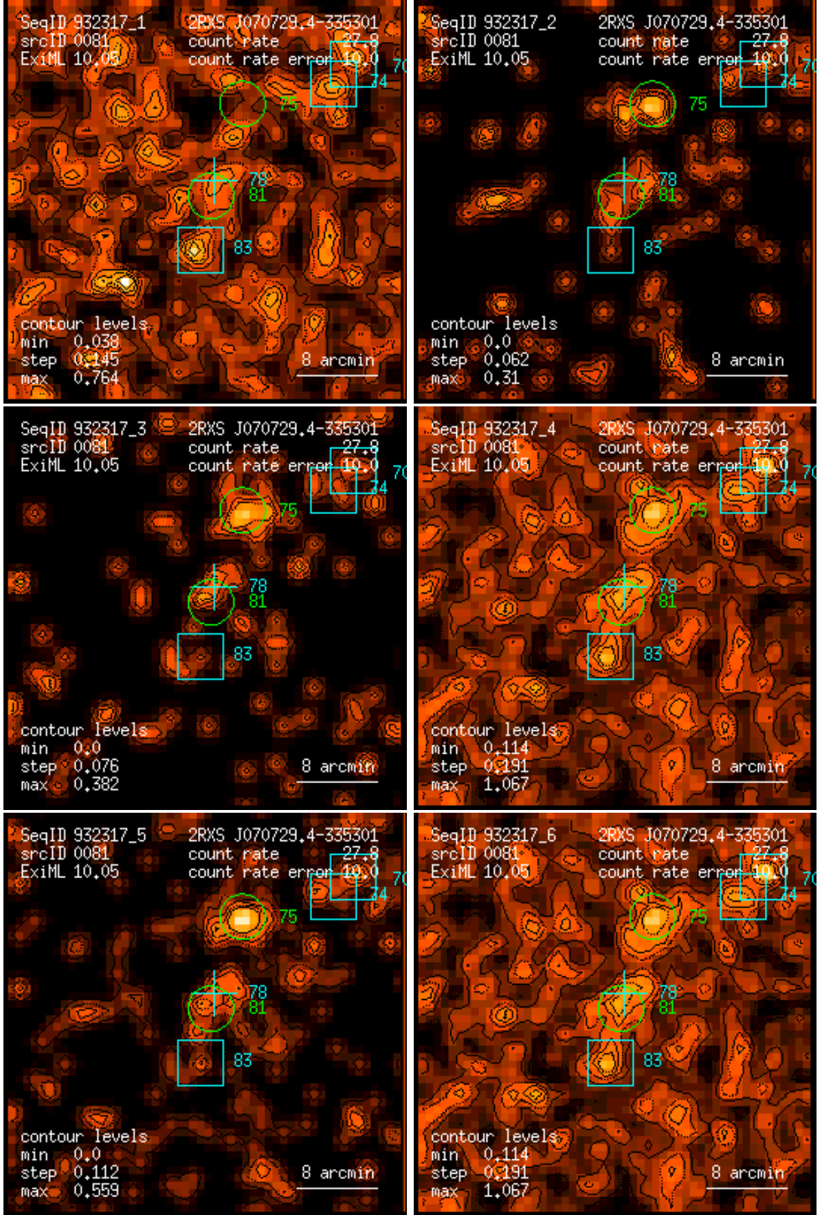
Figure 81: RASS 932317: detection 0081: band rate images, Gaussian filter: (1) PSPC channels 11 – 41, (2) 52 – 90, (3) 91 – 201, (4) 11 – 235, (5) 52 – 201, (6) 11 – 201. Broad band rates in counts/ks. Band rate contour levels in counts/ks/arcmin 2 .
