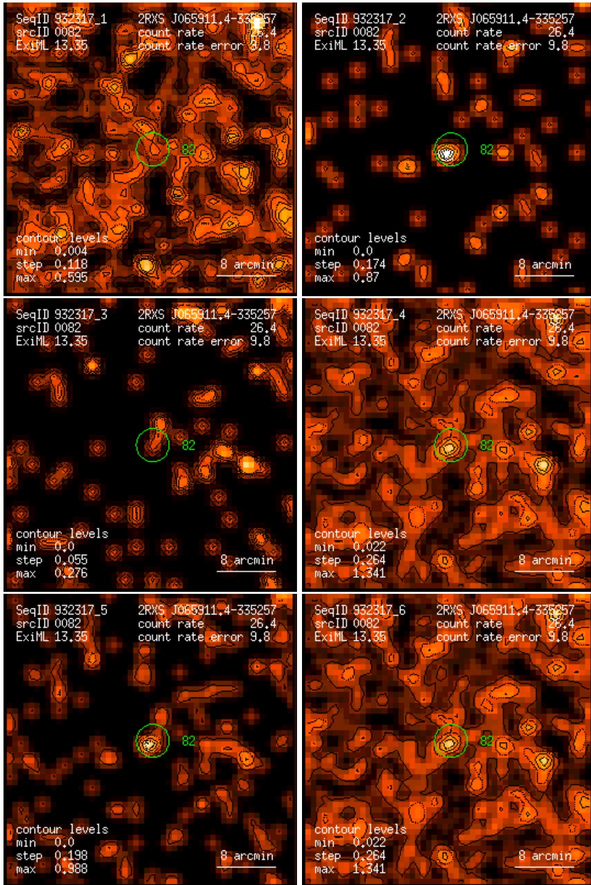
Figure 82: RASS 932317: detection 0082: band rate images, Gaussian filter: (1) PSPC channels 11 – 41, (2) 52 – 90, (3) 91 – 201, (4) 11 – 235, (5) 52 – 201, (6) 11 – 201. Broad band rates in counts/ks. Band rate contour levels in counts/ks/arcmin 2 .
