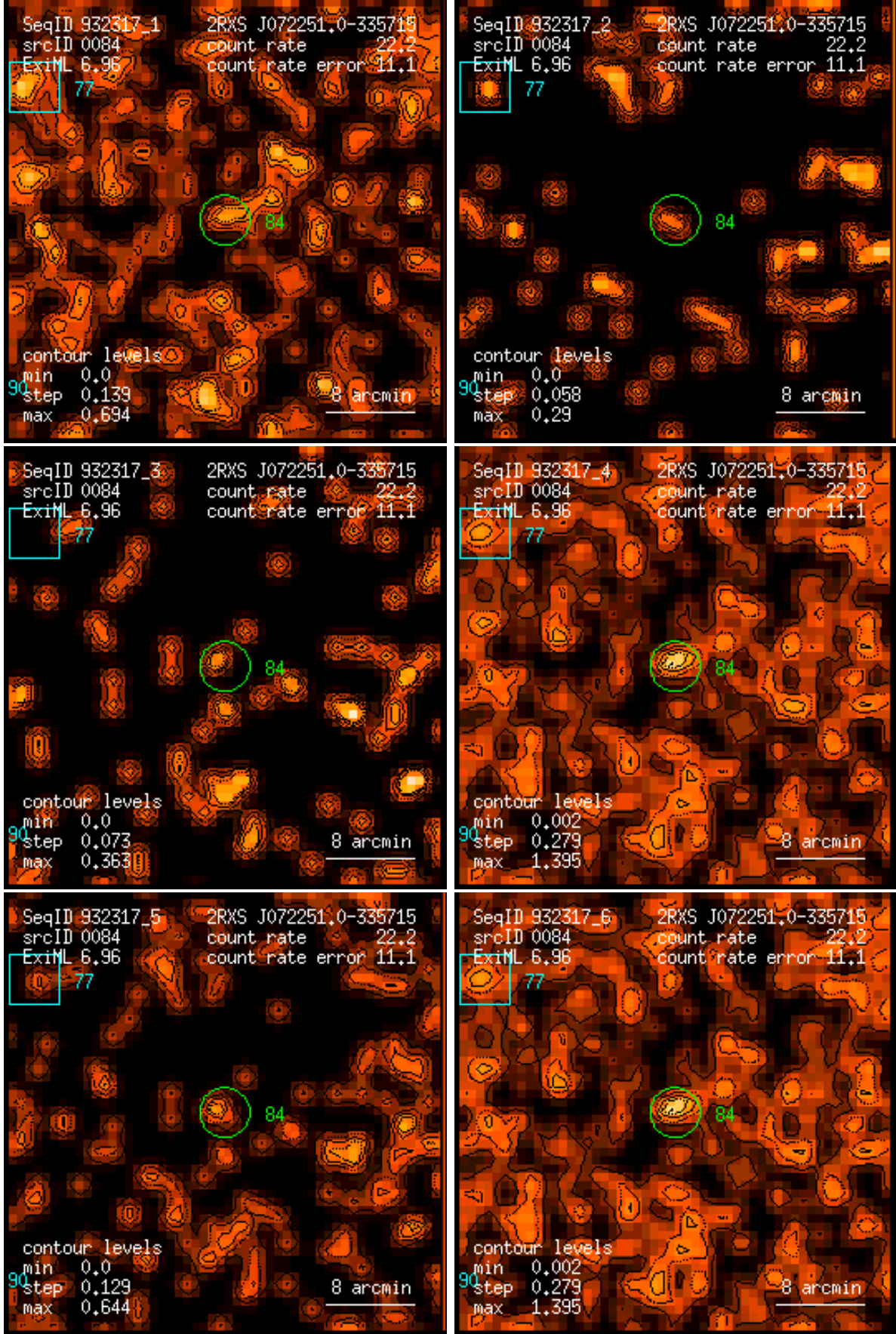
Figure 84: RASS 932317: detection 0084: band rate images, Gaussian filter: (1) PSPC channels 11 – 41, (2) 52 – 90, (3) 91 – 201, (4) 11 – 235, (5) 52 – 201, (6) 11 – 201. Broad band rates in counts/ks. Band rate contour levels in counts/ks/arcmin 2 .
