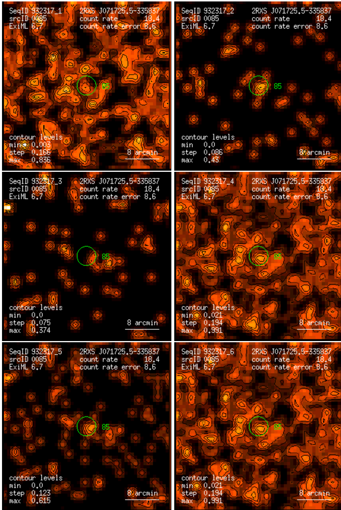
Figure 85: RASS 932317: detection 0085: band rate images, Gaussian filter: (1) PSPC channels 11 – 41, (2) 52 – 90, (3) 91 – 201, (4) 11 – 235, (5) 52 – 201, (6) 11 – 201. Broad band rates in counts/ks. Band rate contour levels in counts/ks/arcmin 2 .
