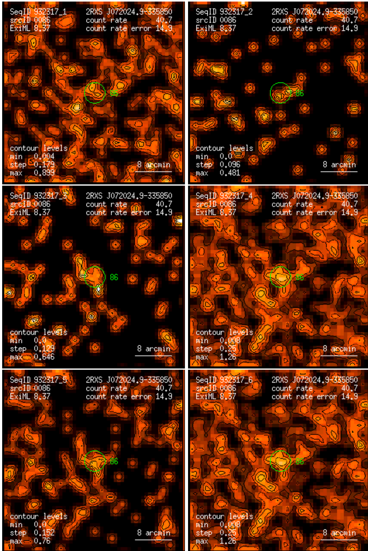
Figure 86: RASS 932317: detection 0086: band rate images, Gaussian filter: (1) PSPC channels 11 – 41, (2) 52 – 90, (3) 91 – 201, (4) 11 – 235, (5) 52 – 201, (6) 11 – 201. Broad band rates in counts/ks. Band rate contour levels in counts/ks/arcmin 2 .
