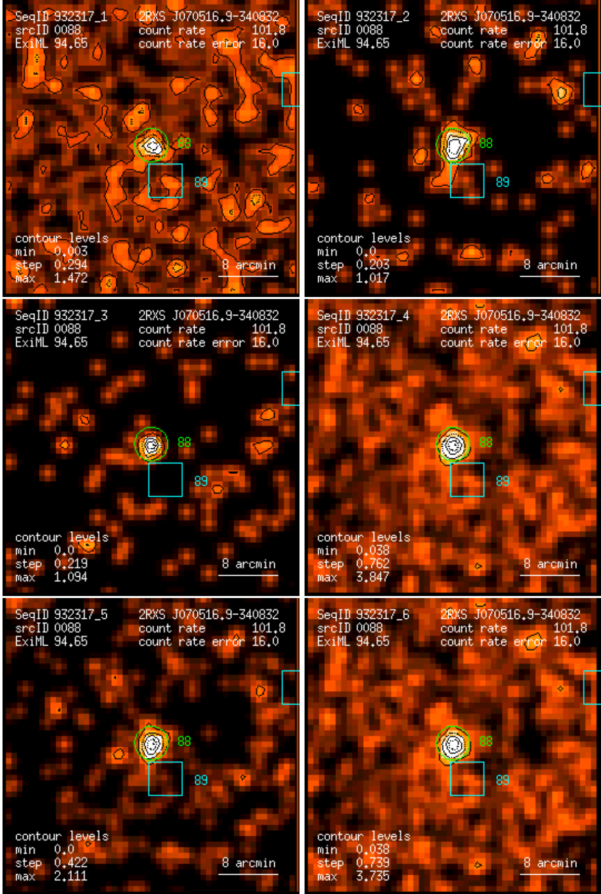
Figure 88: RASS 932317: detection 0088: band rate images, Gaussian filter: (1) PSPC channels 11 – 41, (2) 52 – 90, (3) 91 – 201, (4) 11 – 235, (5) 52 – 201, (6) 11 – 201. Broad band rates in counts/ks. Band rate contour levels in counts/ks/arcmin 2 .
