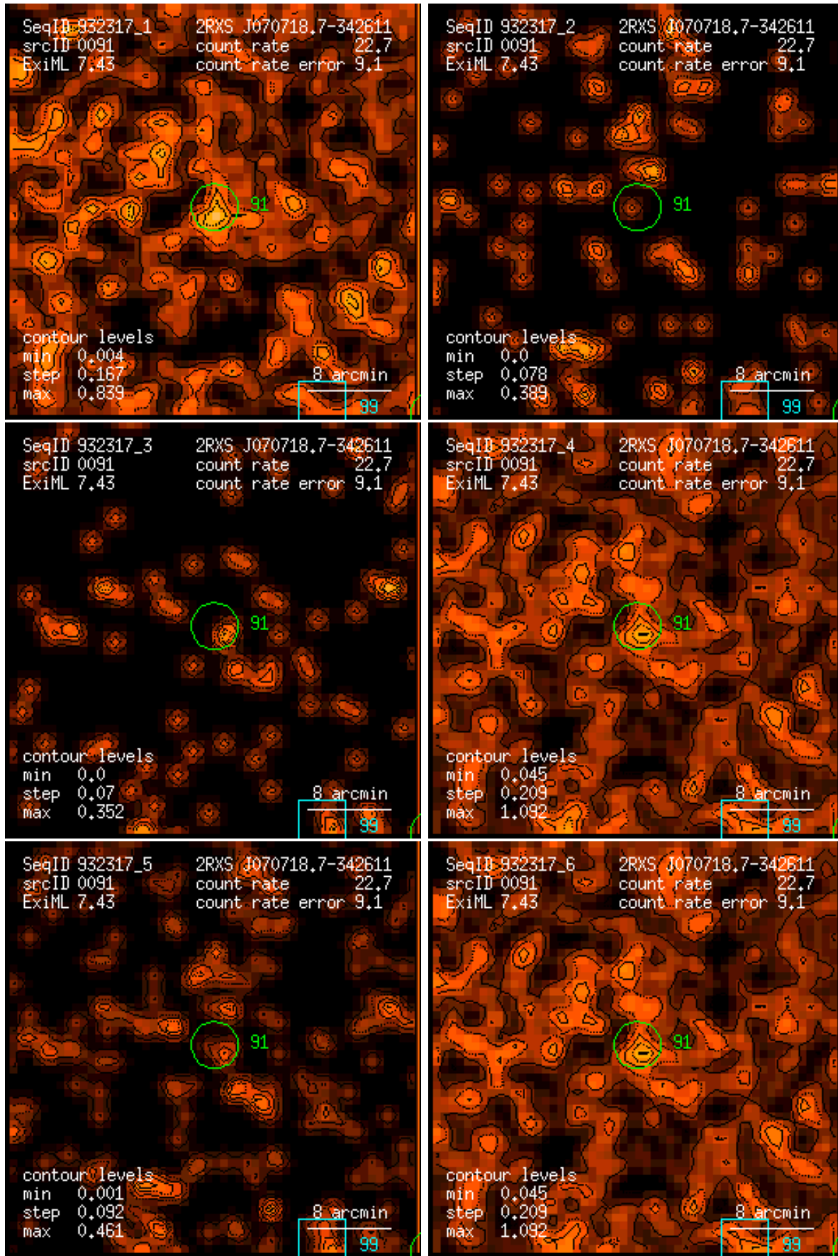
Figure 91: RASS 932317: detection 0091: band rate images, Gaussian filter: (1) PSPC channels 11 – 41, (2) 52 – 90, (3) 91 – 201, (4) 11 – 235, (5) 52 – 201, (6) 11 – 201. Broad band rates in counts/ks. Band rate contour levels in counts/ks/arcmin 2 .
