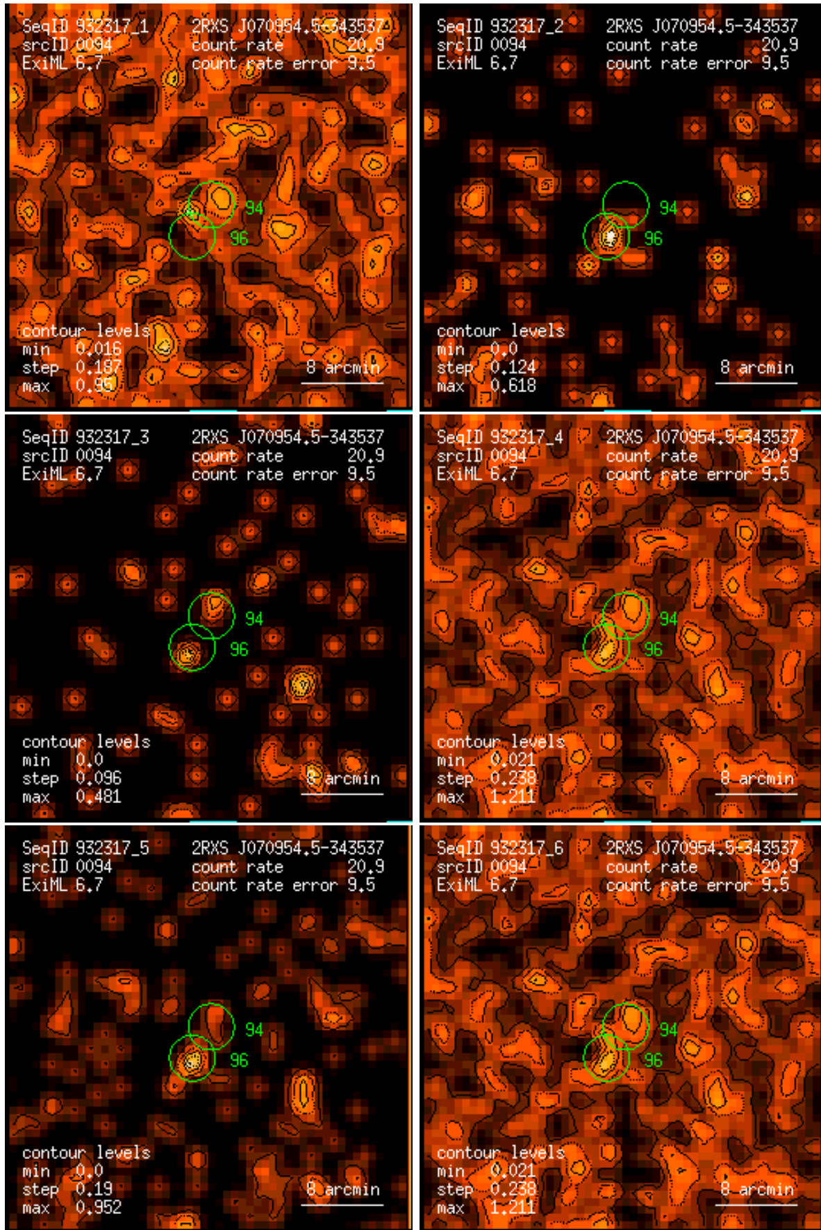
Figure 94: RASS 932317: detection 0094: band rate images, Gaussian filter: (1) PSPC channels 11 – 41, (2) 52 – 90, (3) 91 – 201, (4) 11 – 235, (5) 52 – 201, (6) 11 – 201. Broad band rates in counts/ks. Band rate contour levels in counts/ks/arcmin 2 .
