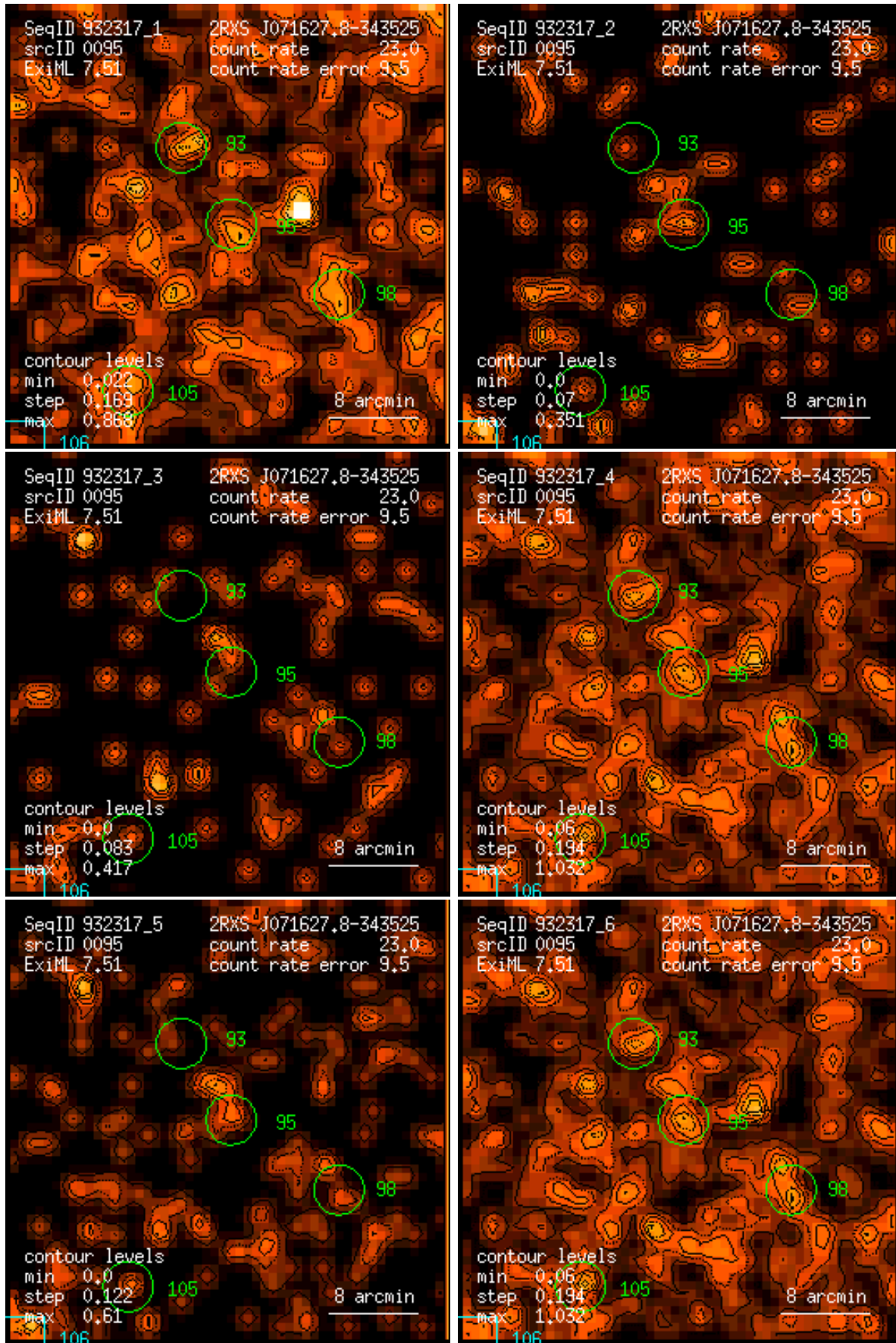
Figure 95: RASS 932317: detection 0095: band rate images, Gaussian filter: (1) PSPC channels 11 – 41, (2) 52 – 90, (3) 91 – 201, (4) 11 – 235, (5) 52 – 201, (6) 11 – 201. Broad band rates in counts/ks. Band rate contour levels in counts/ks/arcmin 2 .
