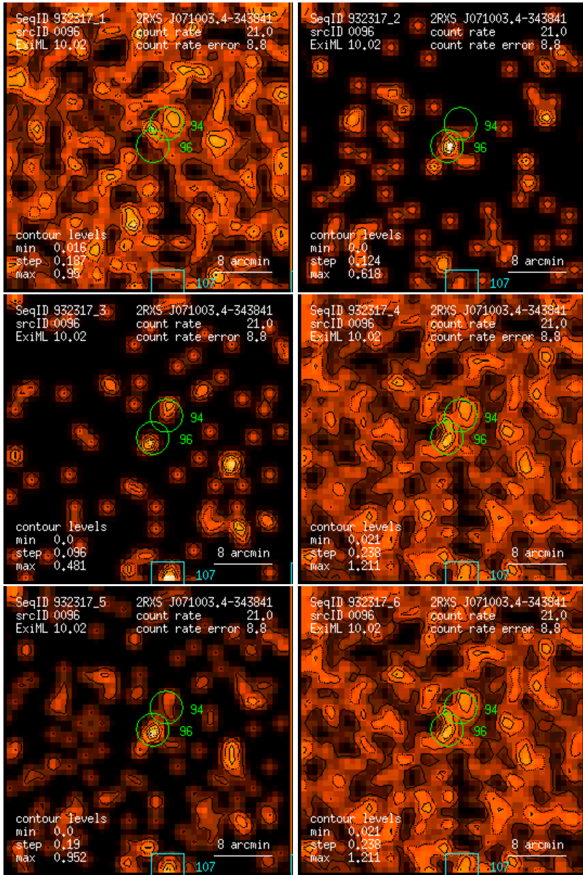
Figure 96: RASS 932317: detection 0096: band rate images, Gaussian filter: (1) PSPC channels 11 – 41, (2) 52 – 90, (3) 91 – 201, (4) 11 – 235, (5) 52 – 201, (6) 11 – 201. Broad band rates in counts/ks. Band rate contour levels in counts/ks/arcmin 2 .
