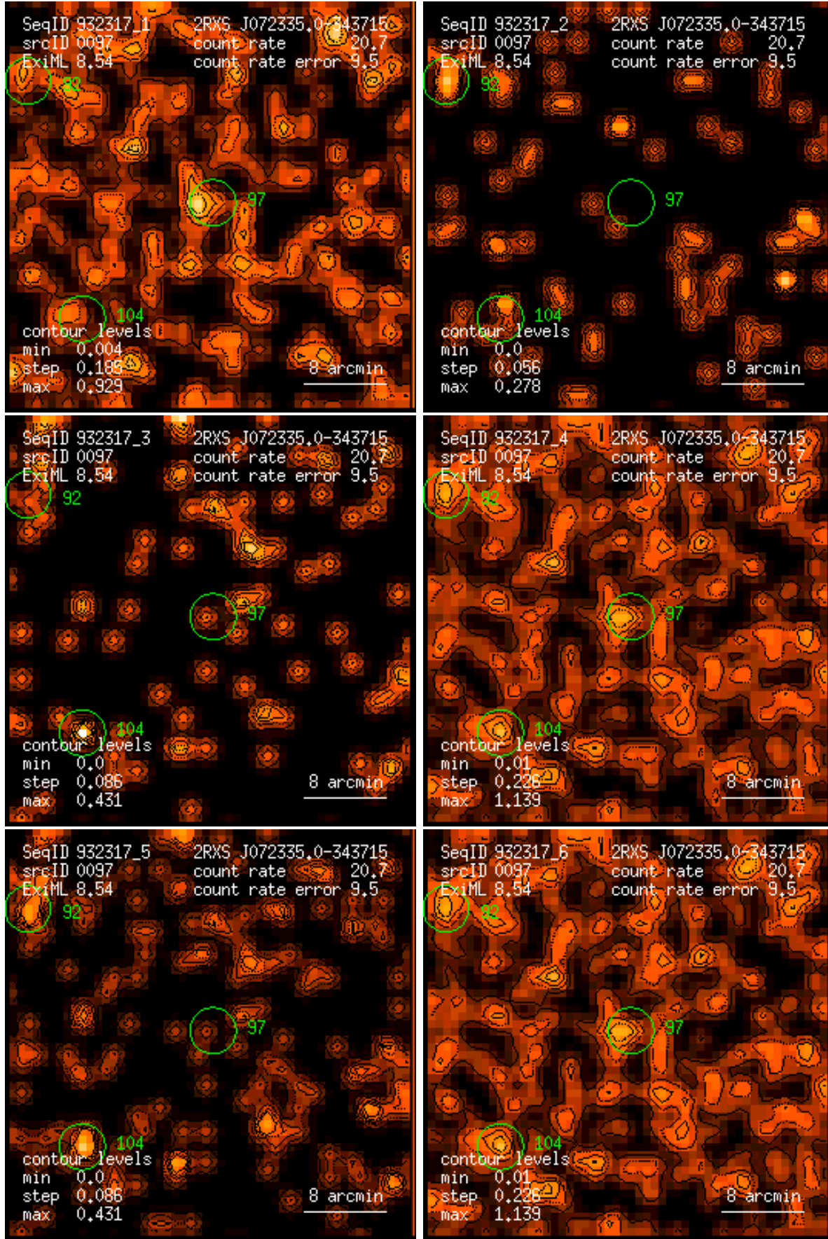
Figure 97: RASS 932317: detection 0097: band rate images, Gaussian filter: (1) PSPC channels 11 – 41, (2) 52 – 90, (3) 91 – 201, (4) 11 – 235, (5) 52 – 201, (6) 11 – 201. Broad band rates in counts/ks. Band rate contour levels in counts/ks/arcmin 2 .
