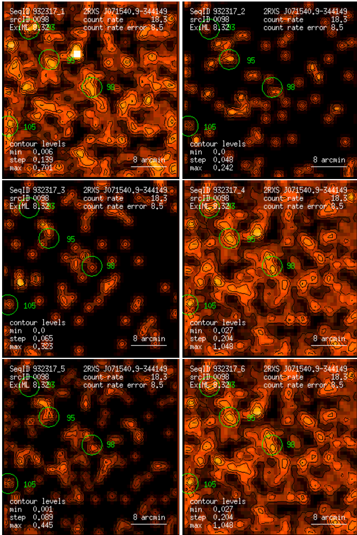
Figure 98: RASS 932317: detection 0098: band rate images, Gaussian filter: (1) PSPC channels 11 – 41, (2) 52 – 90, (3) 91 – 201, (4) 11 – 235, (5) 52 – 201, (6) 11 – 201. Broad band rates in counts/ks. Band rate contour levels in counts/ks/arcmin 2 .
